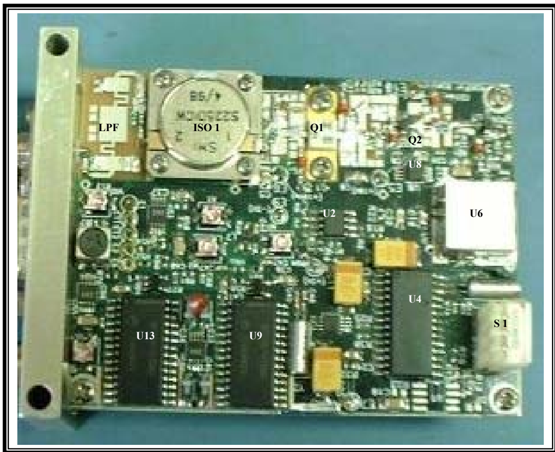
AT-100S RF Board
