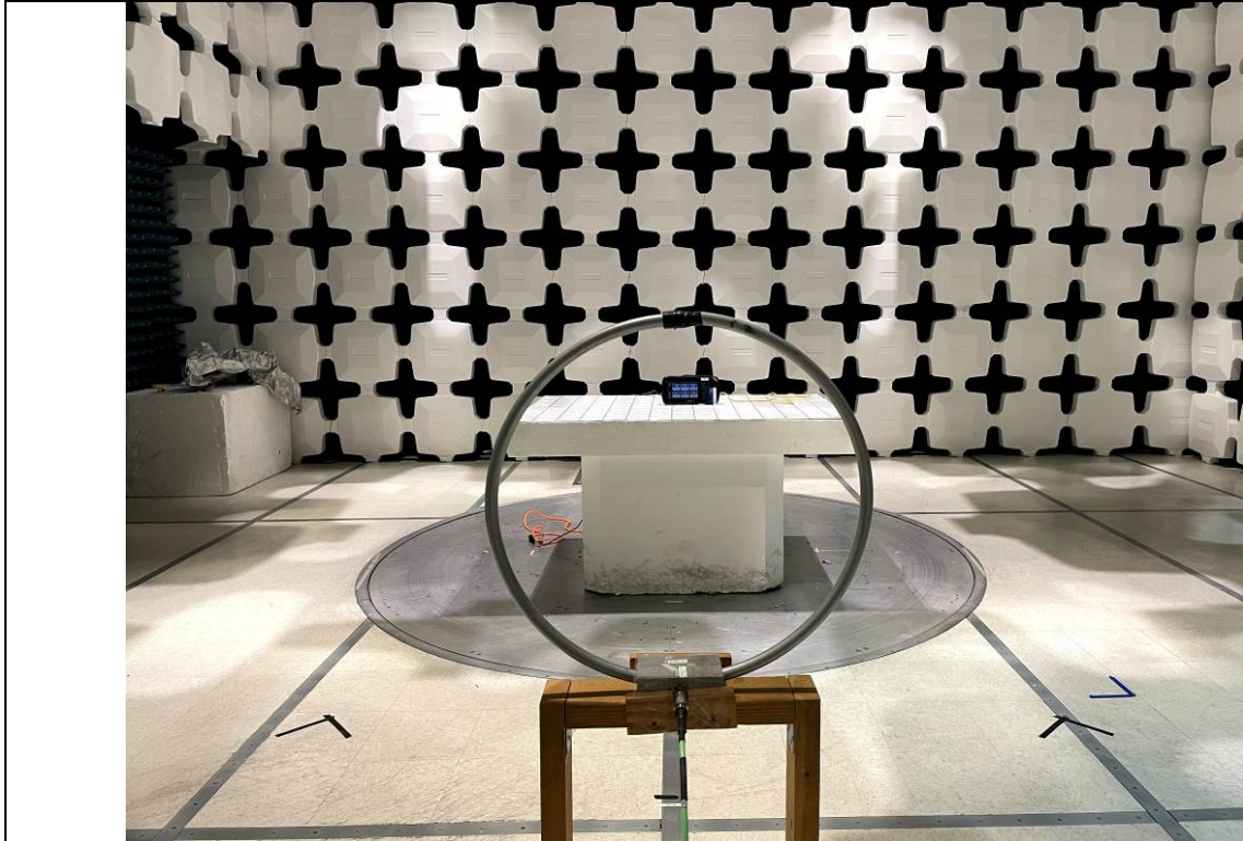
Radiated Emission Test below 30MHz Front View
