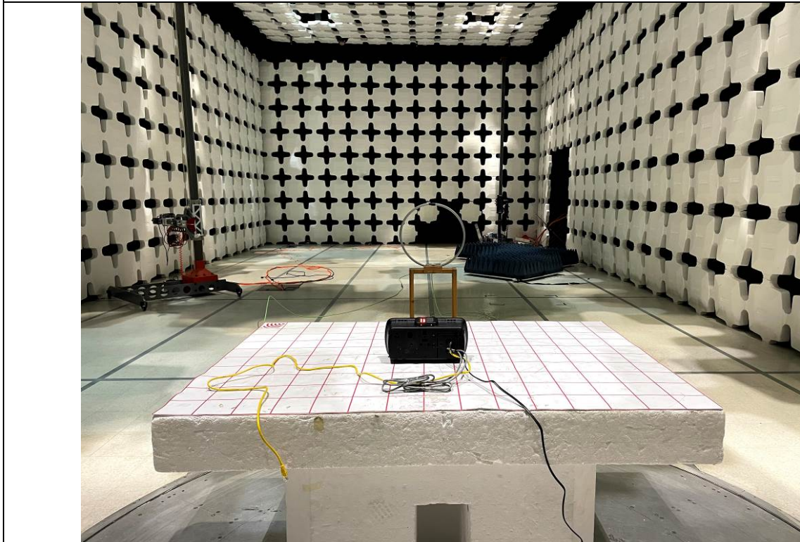
Radiated Emission Test below 30MHz Rear View
