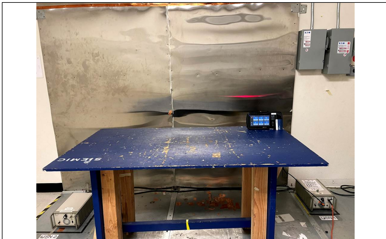
Conducted Emission Test Front View
