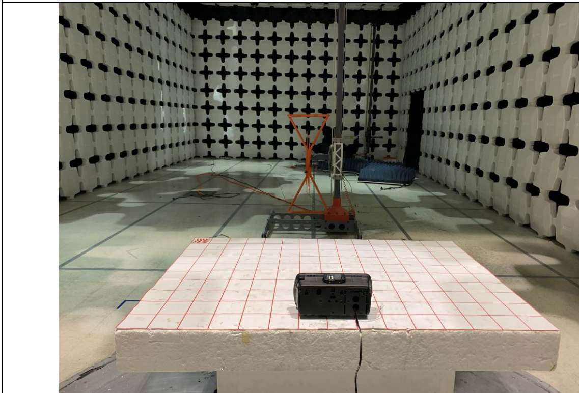
Radiated Emission Test 30MHz-1GHz Rear View
