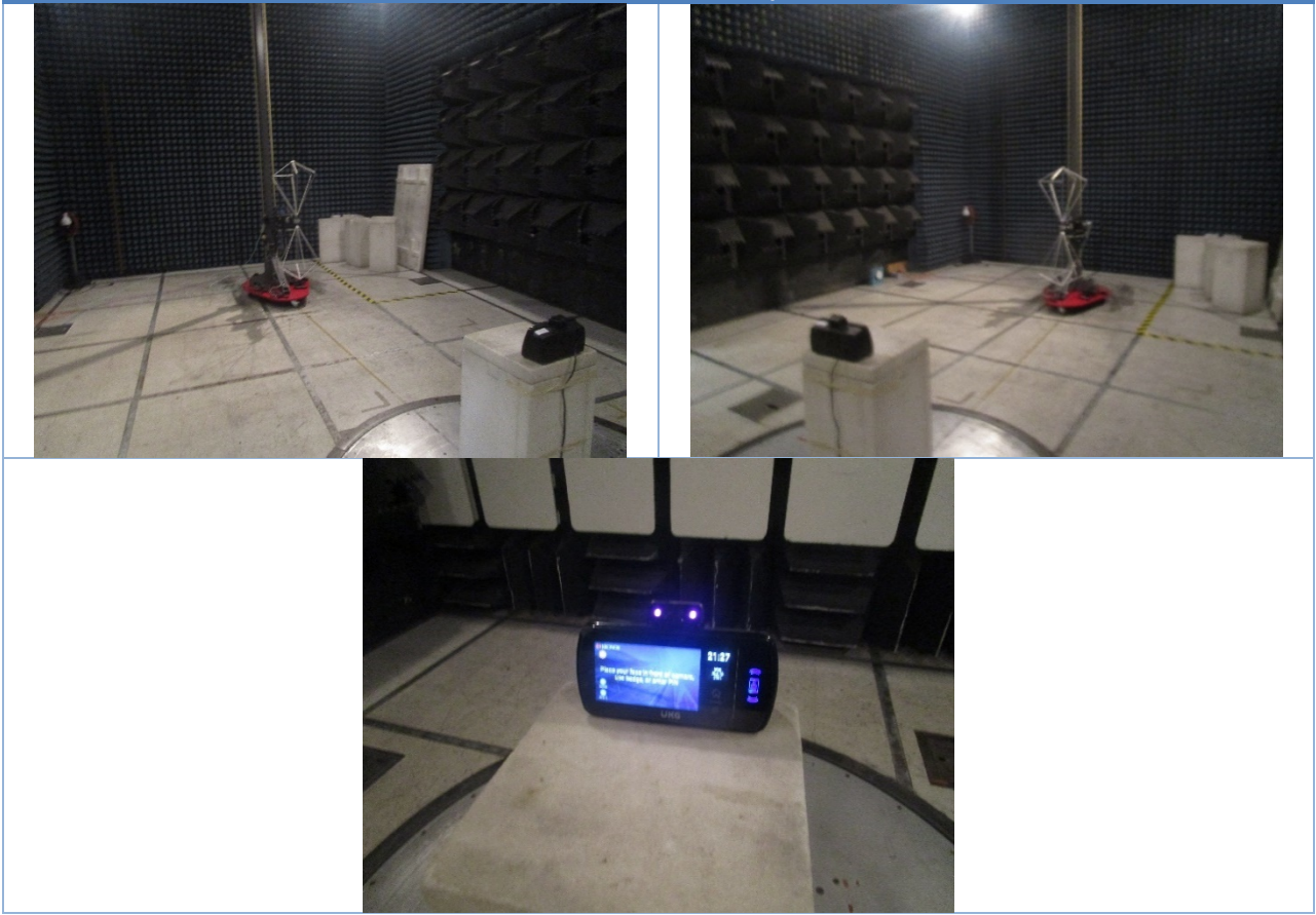
Radiated Emissions: FCC 15.209 | 30-1000 MHz
