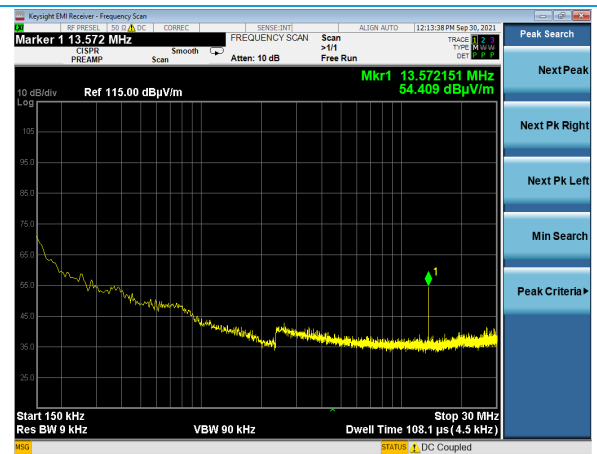
Parallel: 0.15 – 30 MHz
