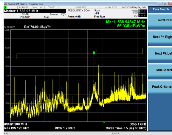
200 – 1000 MHz: Horizontal Polarity
