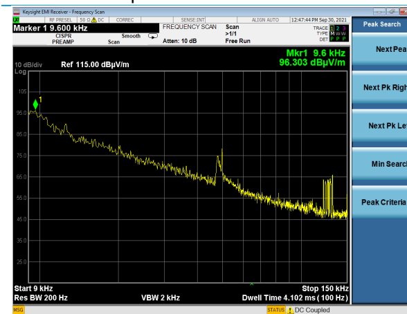
Skew: 9 – 150 kHz
