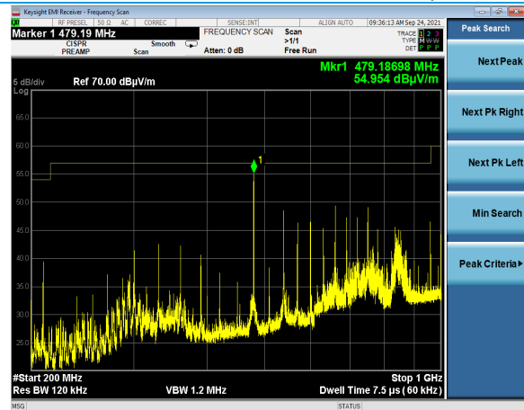
200 – 1000 MHz: Vertical Polarity
