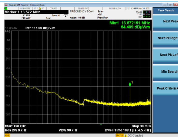
Parallel: 0.15 – 30 MHz
