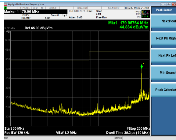
30 – 200 MHz: Horizontal Polarity
