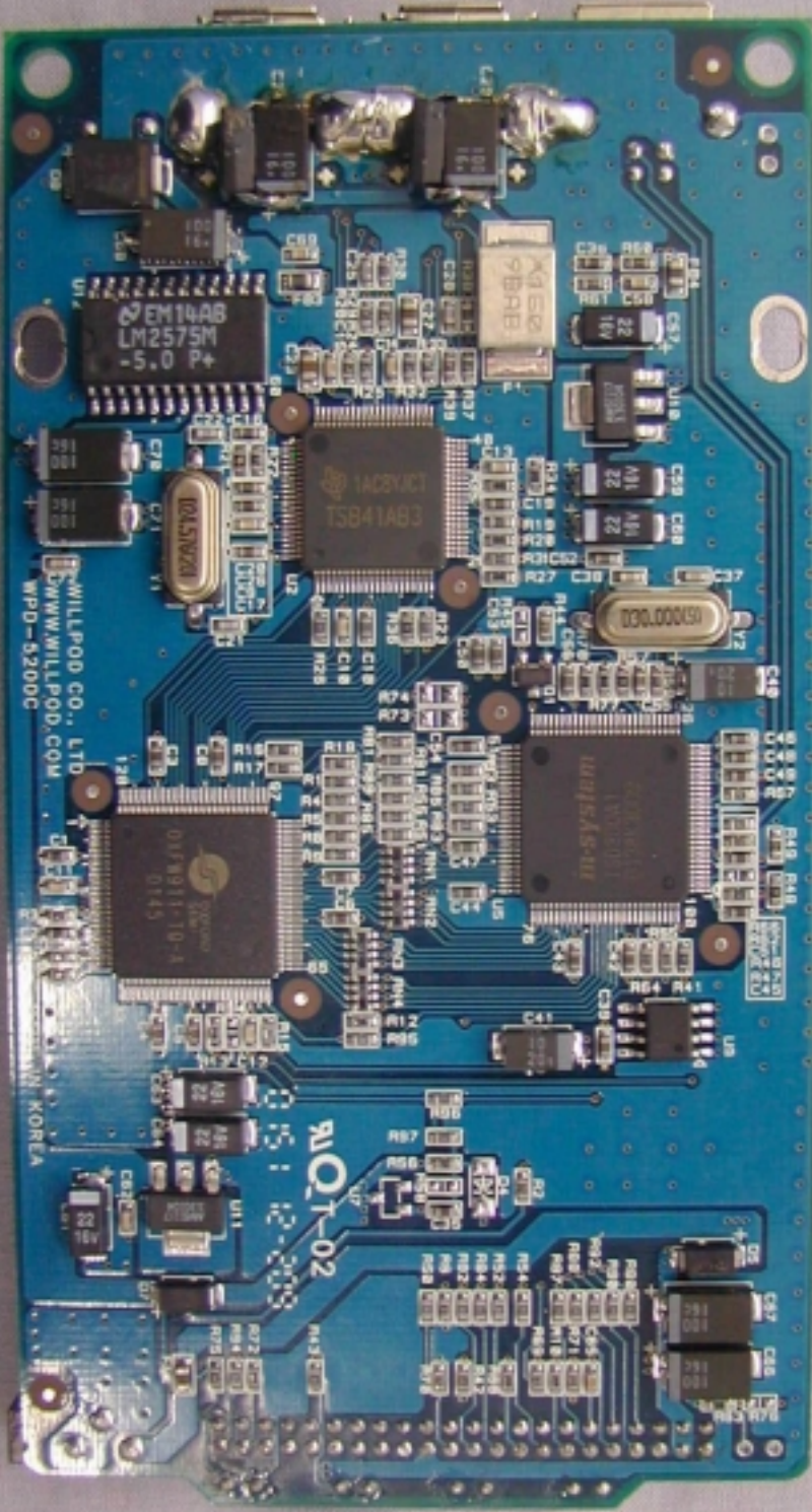
<FRONT VIEW OF MAIN BOARD>
