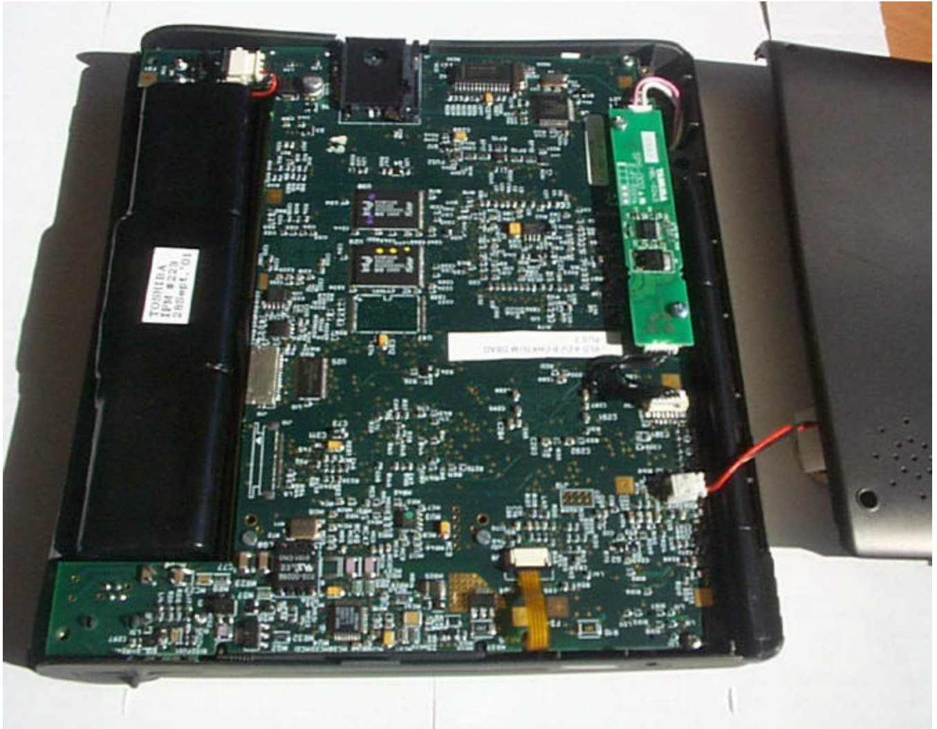
PARTIALLY DISASSEMBLED
