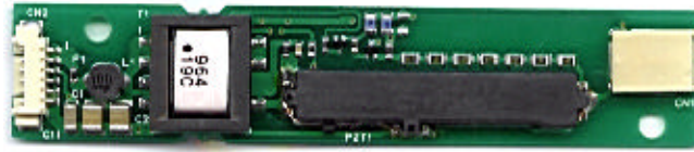
INVERTER BOARD SIDE 1
