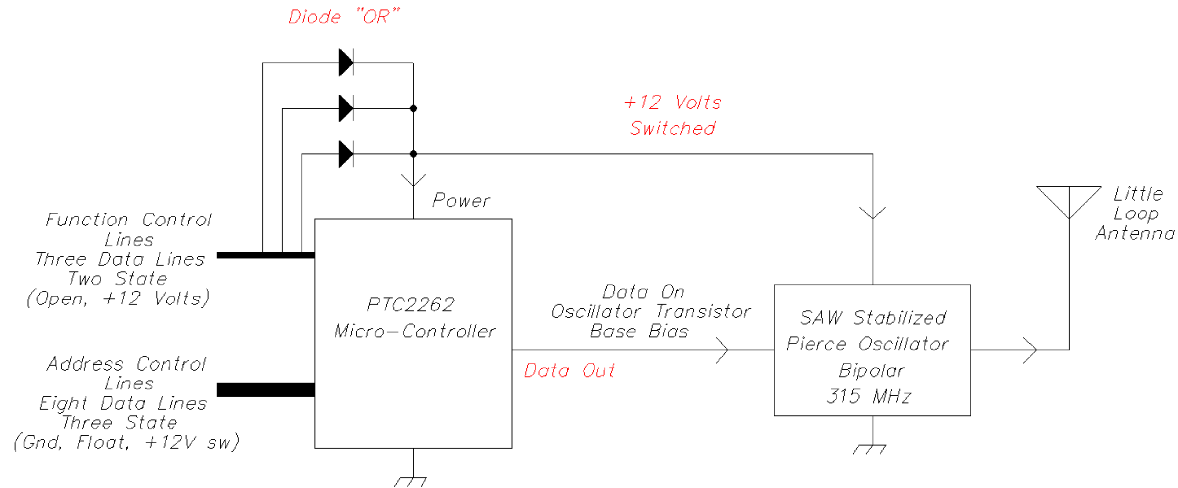
Basic SALIO Transmitter Block Diagram
