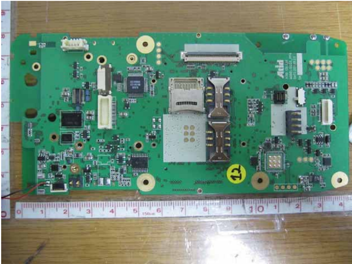
Main board
