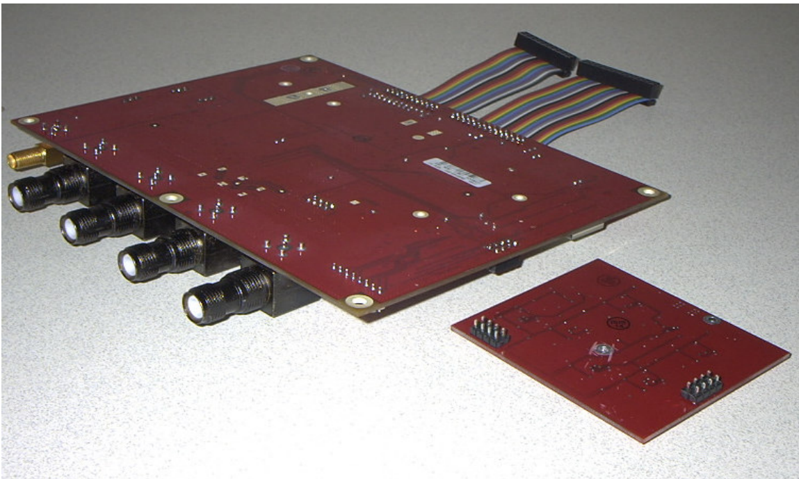
RF Internal Bottom, With Daughter PCA NOT Installed
