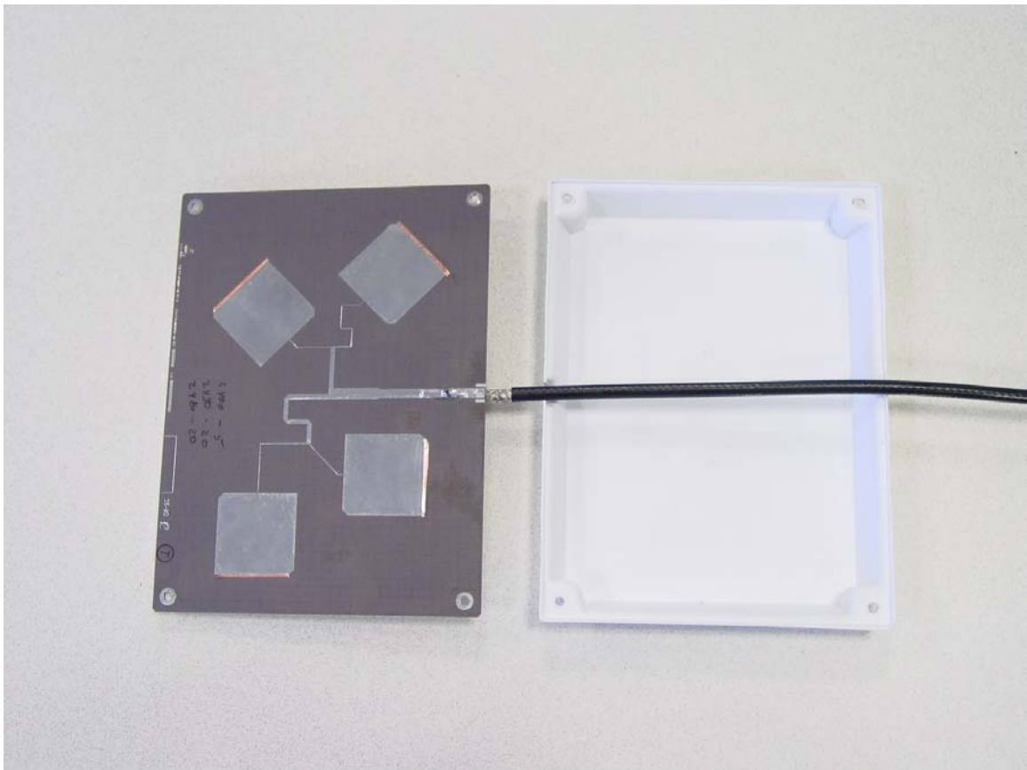
Alien Antenna Assembly
