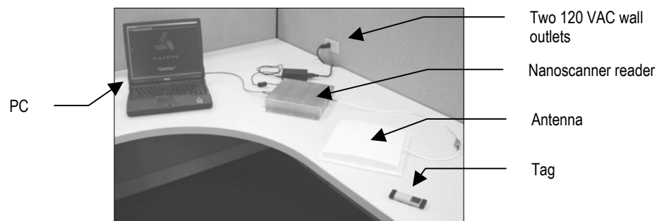
Typical reader system benchtest set-up.
