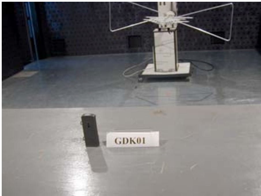
Photo 2: Radiated set-up
