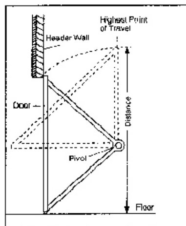
One-piece door without track: pivot hardware
