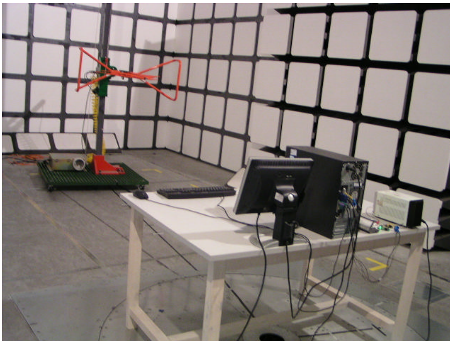
Transmitting Mode: Radiated Emission - Rear View (30 MHz-1000MHz)
