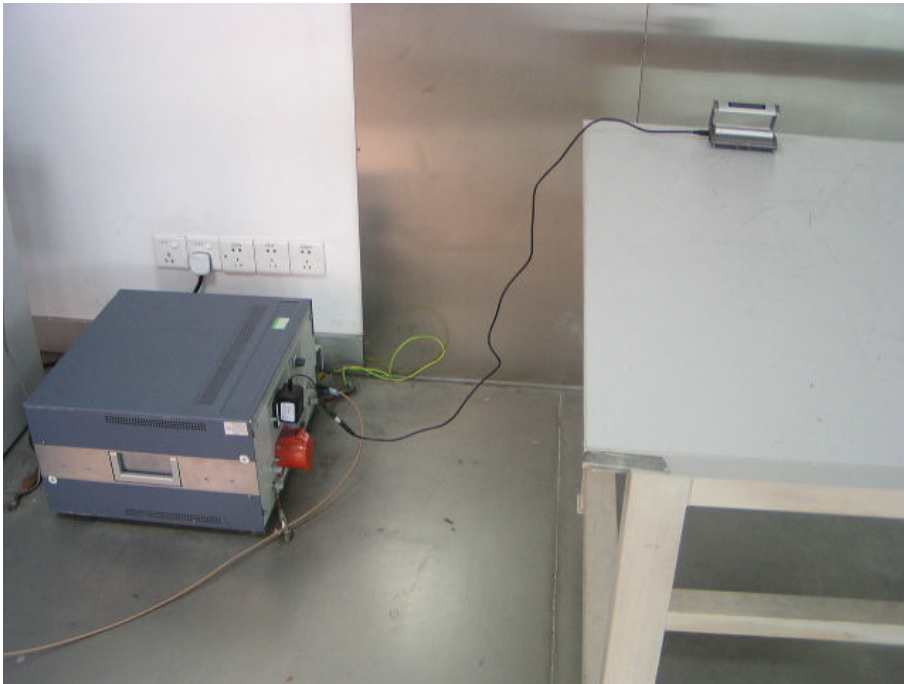
Charging Mode: Conducted Emissions-Front View
