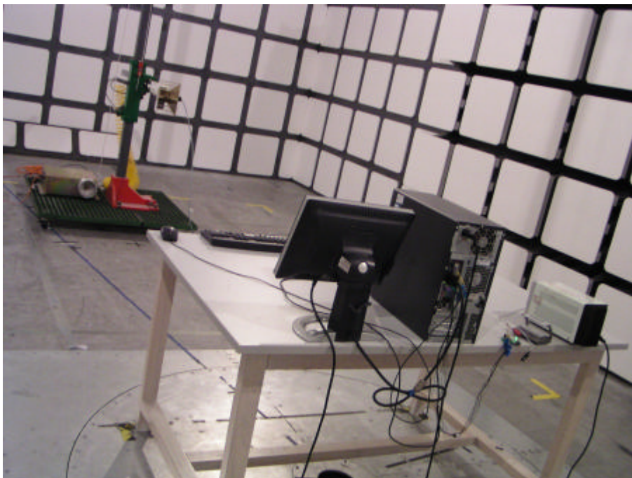
Transmitting Mode: Radiated Emission – Rear View (1000-25000MHz)
