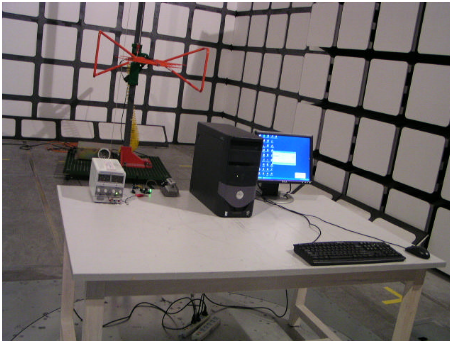
Transmitting Mode: Radiated Emission - Front View (30 MHz-1000MHz)
