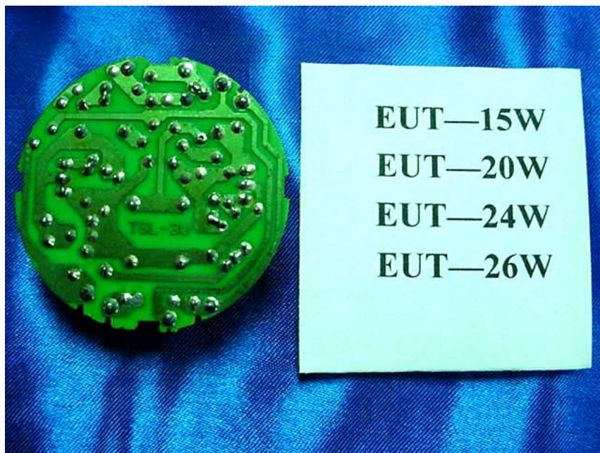
Figure 11 M/N: EUT Series Main Board, Component Side
