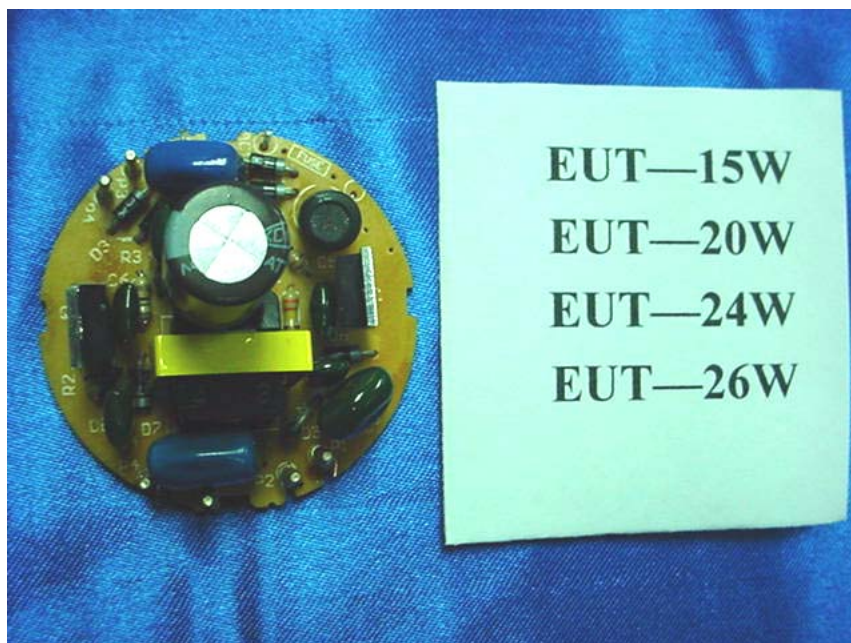
Figure 10 M/N: EUT Series Main Board, Component Side
