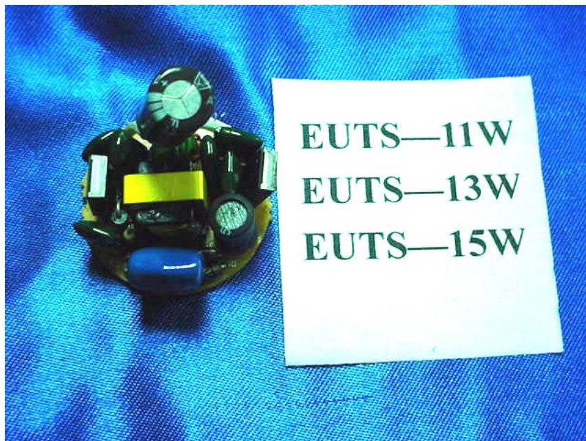
Figure 6 M/N: EUTS Series Main Board, Component Side
