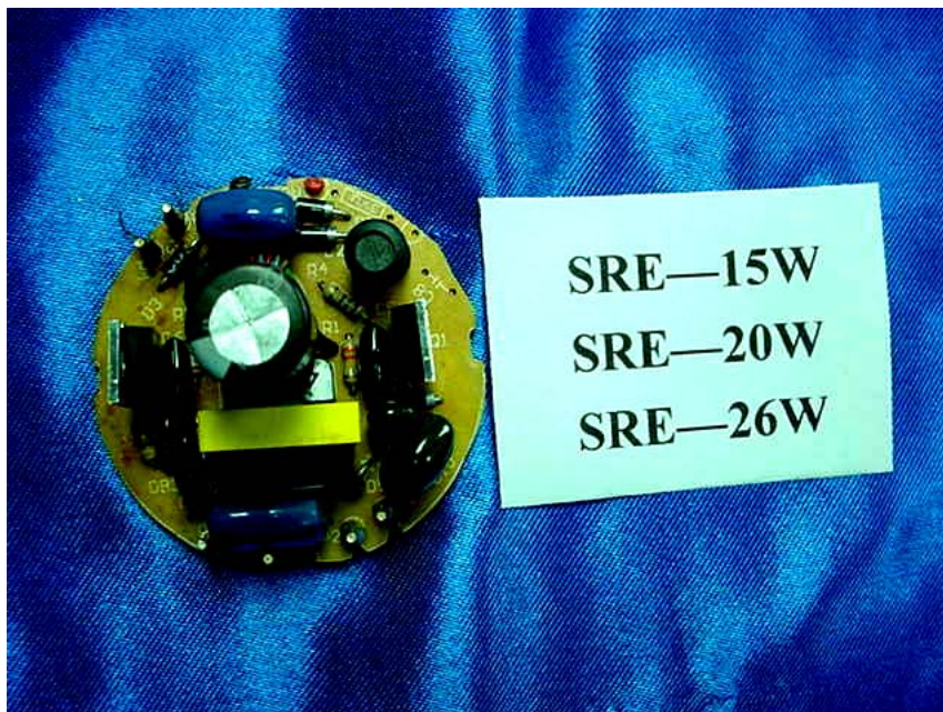
Figure 12 M/N: SRE Series Main Board, Component Side
