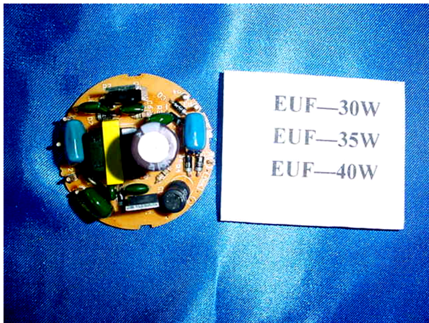
Figure 14 M/N: EUF Series Main Board, Component Side
