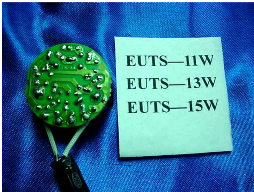
Figure 7 M/N: EUTS Series Main Board, Component Side
