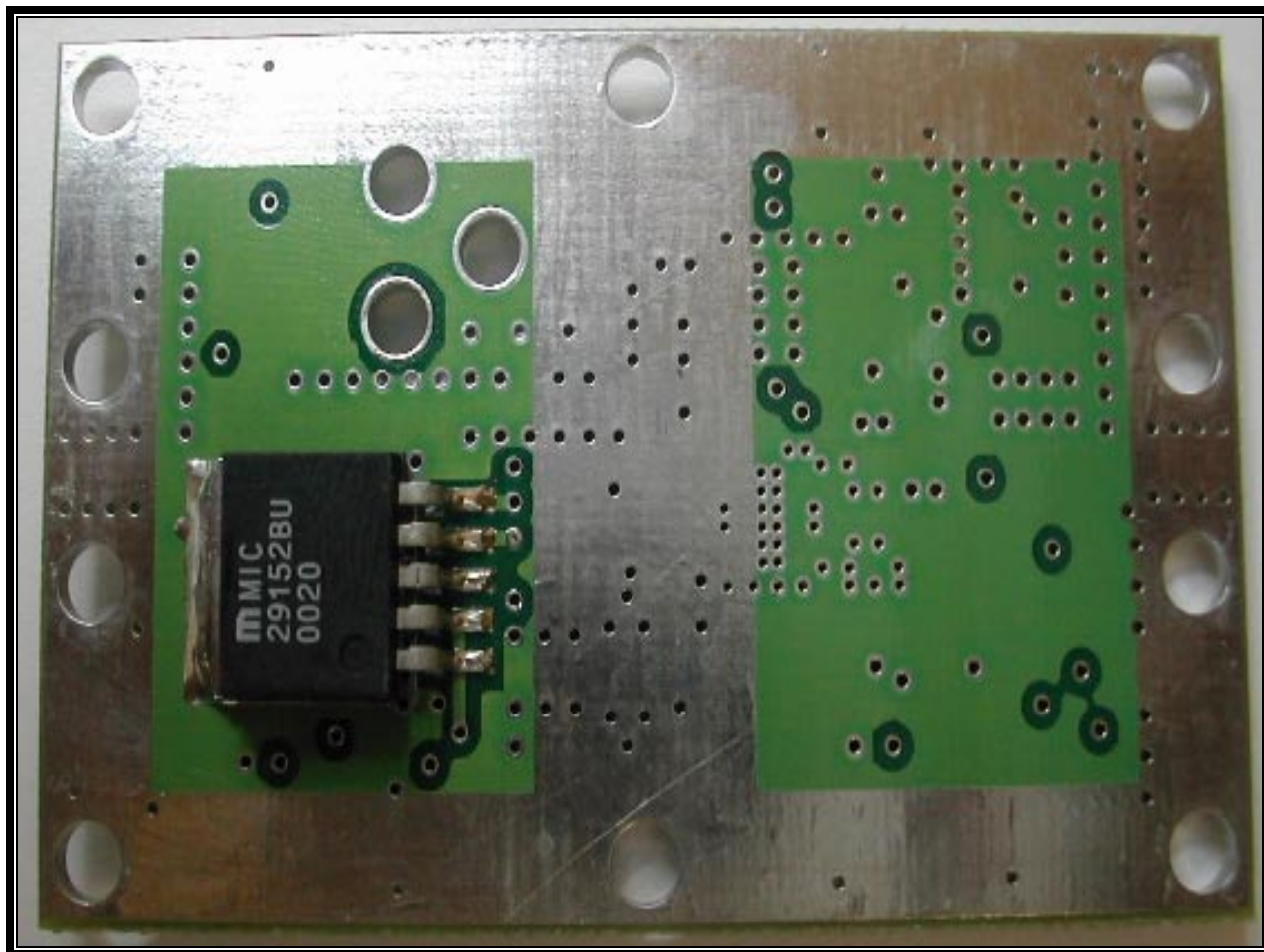
PHOTOGRAPH 22: REAR VIEW PCB FROM 500mW AMPLIFIER
