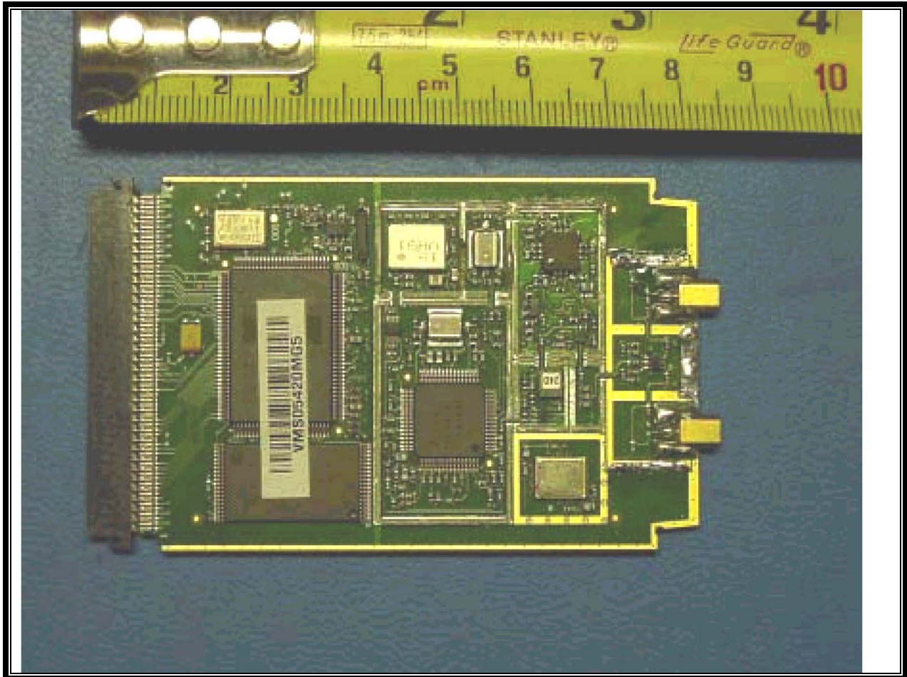
PHOTOGRAPH 19: BACK VIEW OF PCB WITHOUT SHIELD
