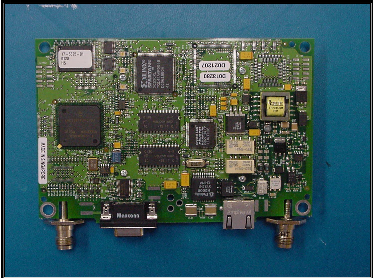
PHOTOGRAPH 14: FRONT VIEW DIGITAL PART OF THE ACCESS POINT
