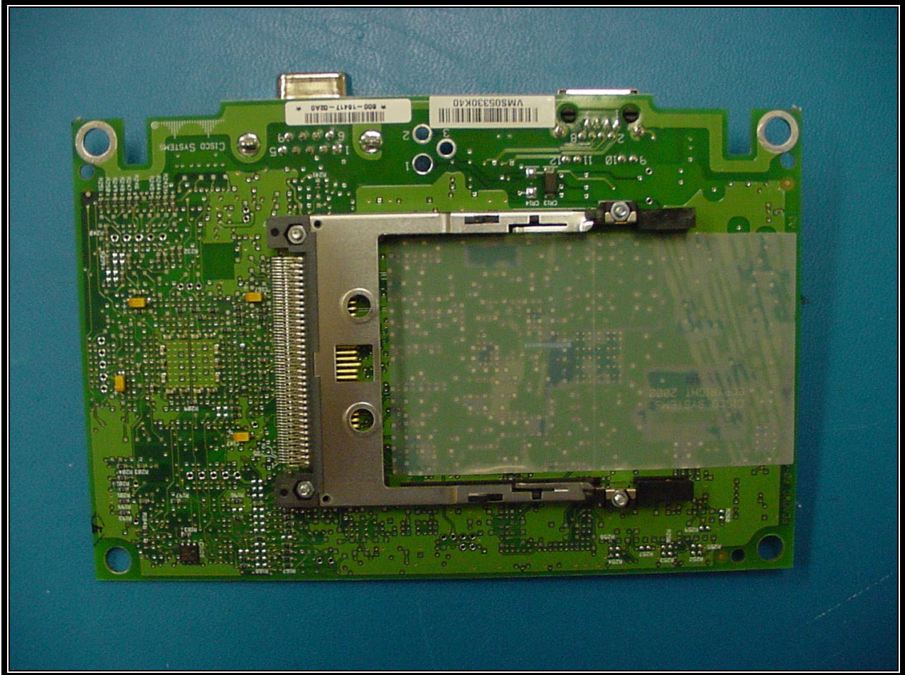
PHOTOGRAPH 15: REAR VIEW DIGITAL PART OF THE ACCESS POINT
