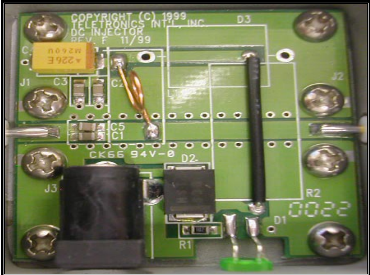
PHOTOGRAPH 20: FRONT VIEW PCB FROM DC INJECTOR
