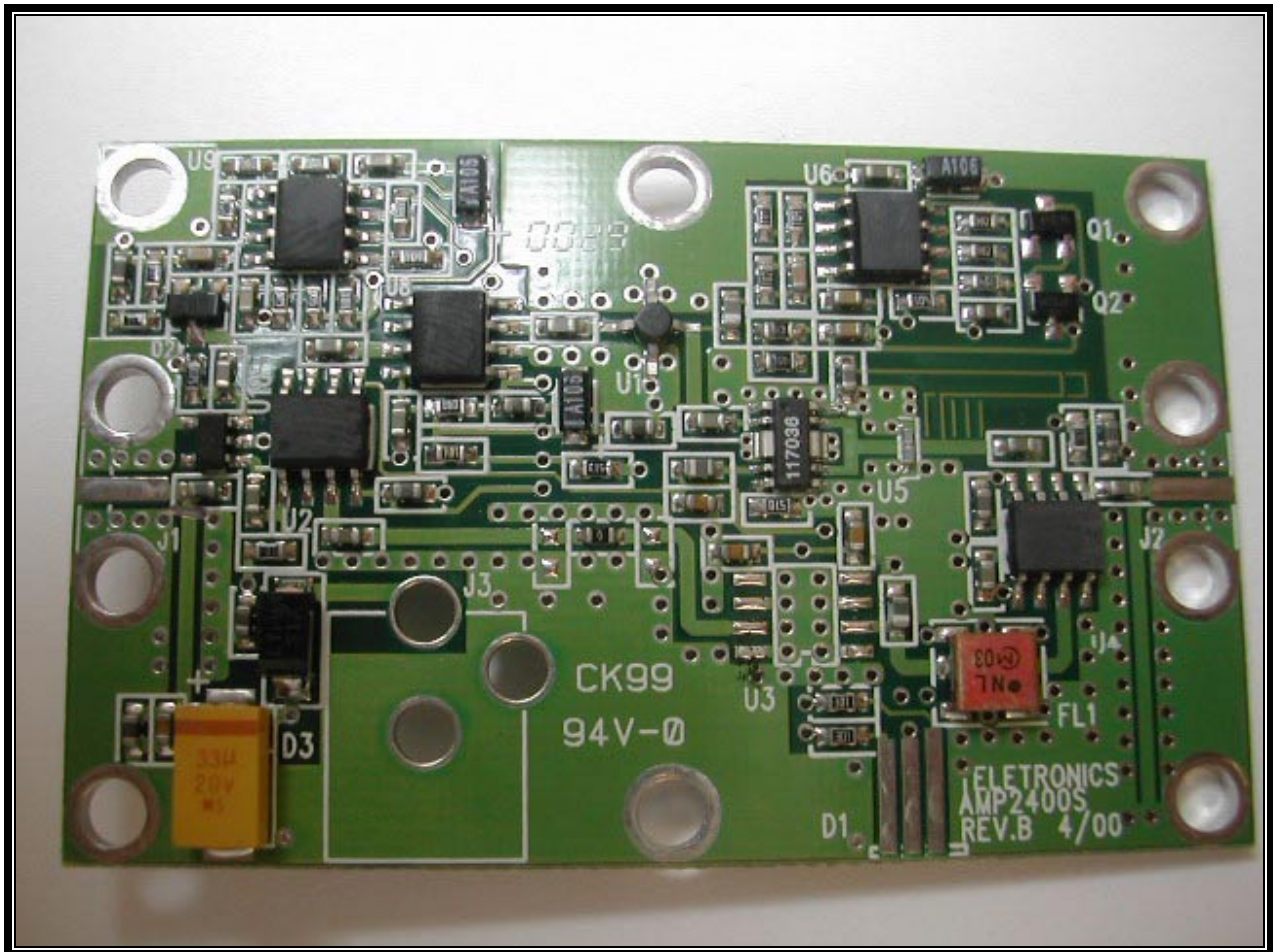
PHOTOGRAPH 21: FRONT VIEW PCB FROM 500mW AMPLIFIER
