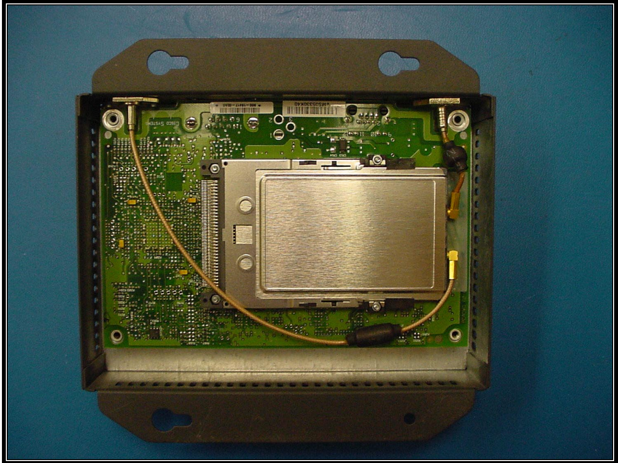
PHOTOGRAPH 13: INSIDE VIEW OF THE ACCESS POINT
