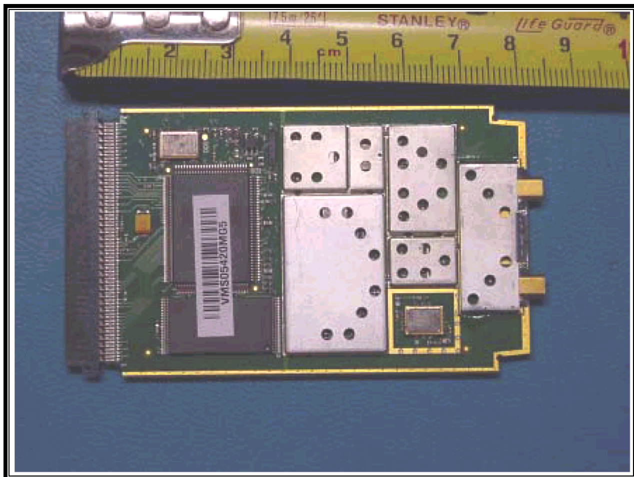
PHOTOGRAPH 18: BACK VIEW OF PCB WITH SHIELD
