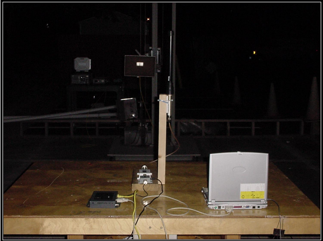
PHOTOGRAPH 4: RADIATED EMISSION REAR VIEW, WORST CASE CONFIGURATION - 6dBi
