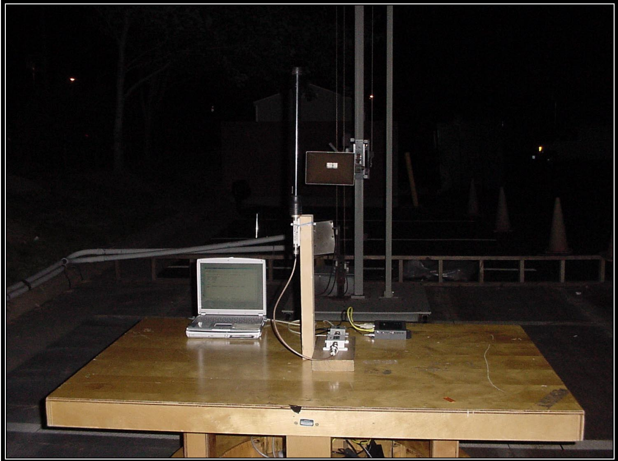
PHOTOGRAPH 6: RADIATED EMISSION REAR VIEW, WORST CASE CONFIGURATION - 9 dBi
