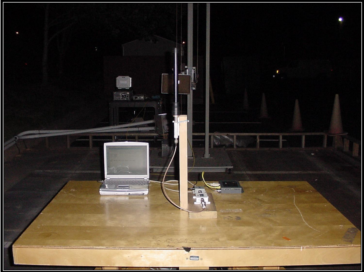
PHOTOGRAPH 3: RADIATED EMISSION FRONT VIEW, WORST CASE CONFIGURATION - 6dBi
