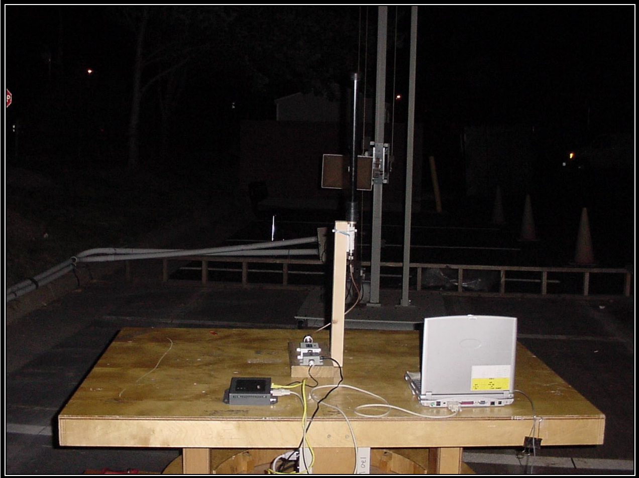
PHOTOGRAPH 5: RADIATED EMISSION FRONT VIEW, WORST CASE CONFIGURATION - 9dBi
