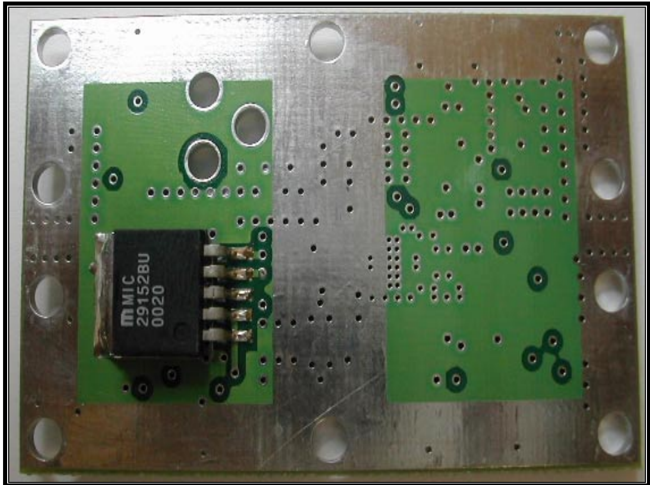
PHOTOGRAPH 25: BACK VIEW PCB FROM 1W AMPLIFIER
