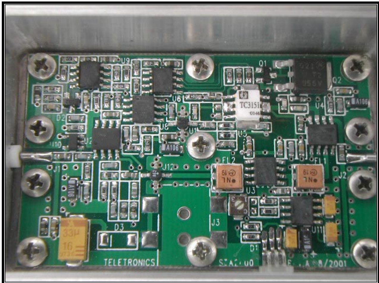
PHOTOGRAPH 24: FRONT VIEW PCB FROM 1W AMPLIFIER
