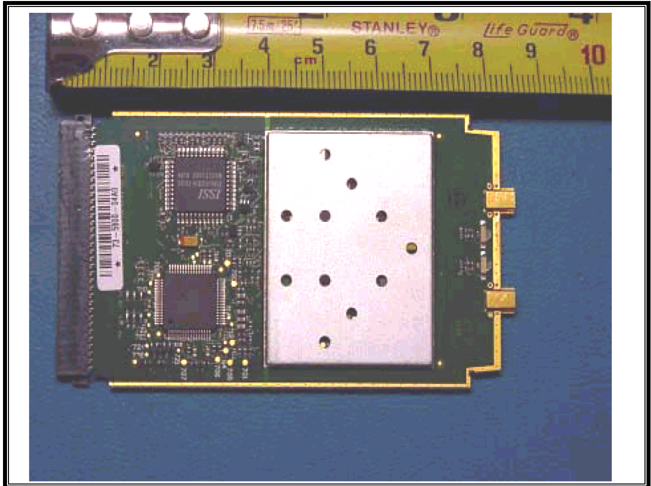
PHOTOGRAPH 16: FRONT VIEW OF PCB WITH SHIELD
