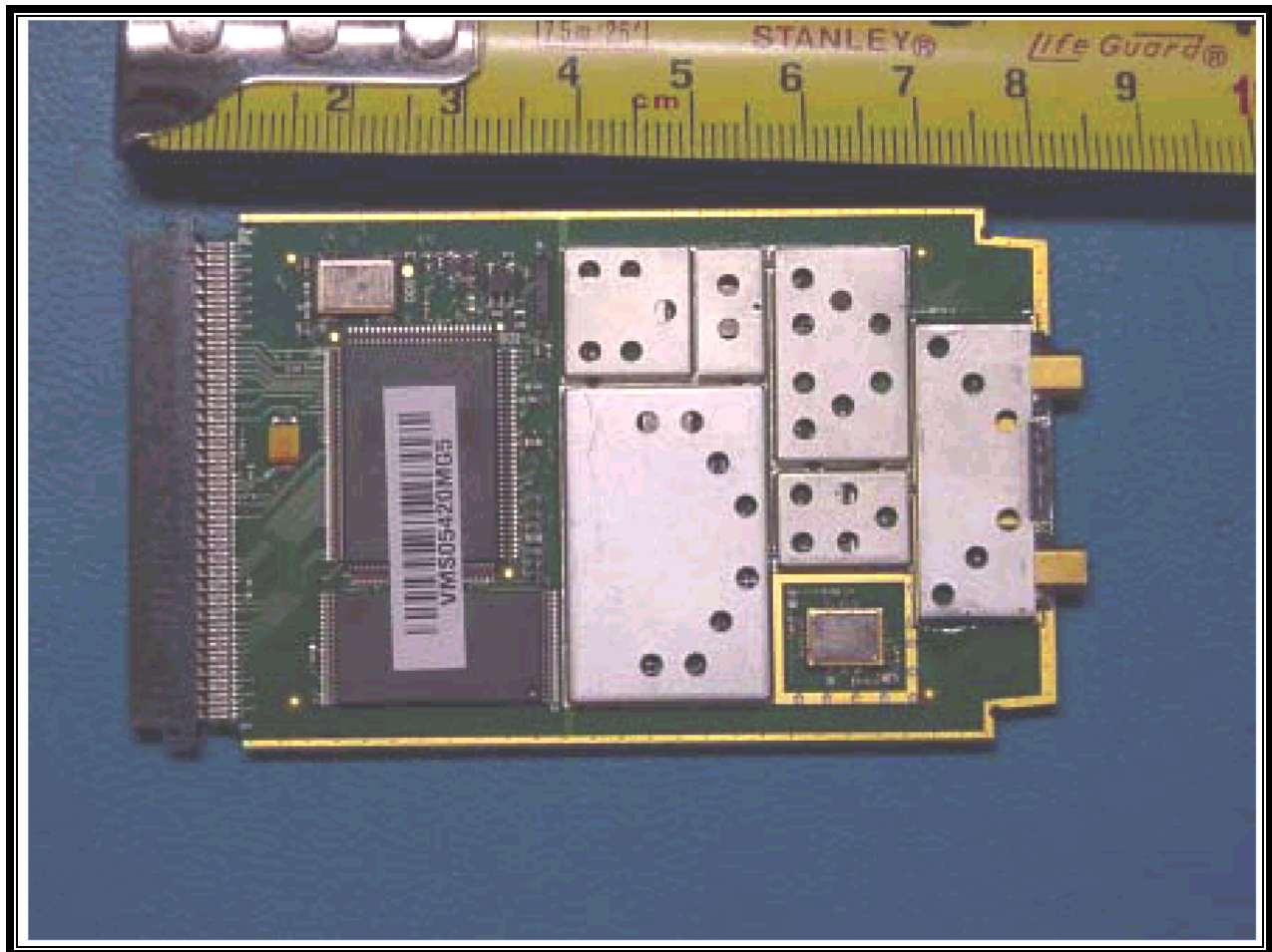
PHOTOGRAPH 18: BACK VIEW OF THE PCB WITH SHIELD
