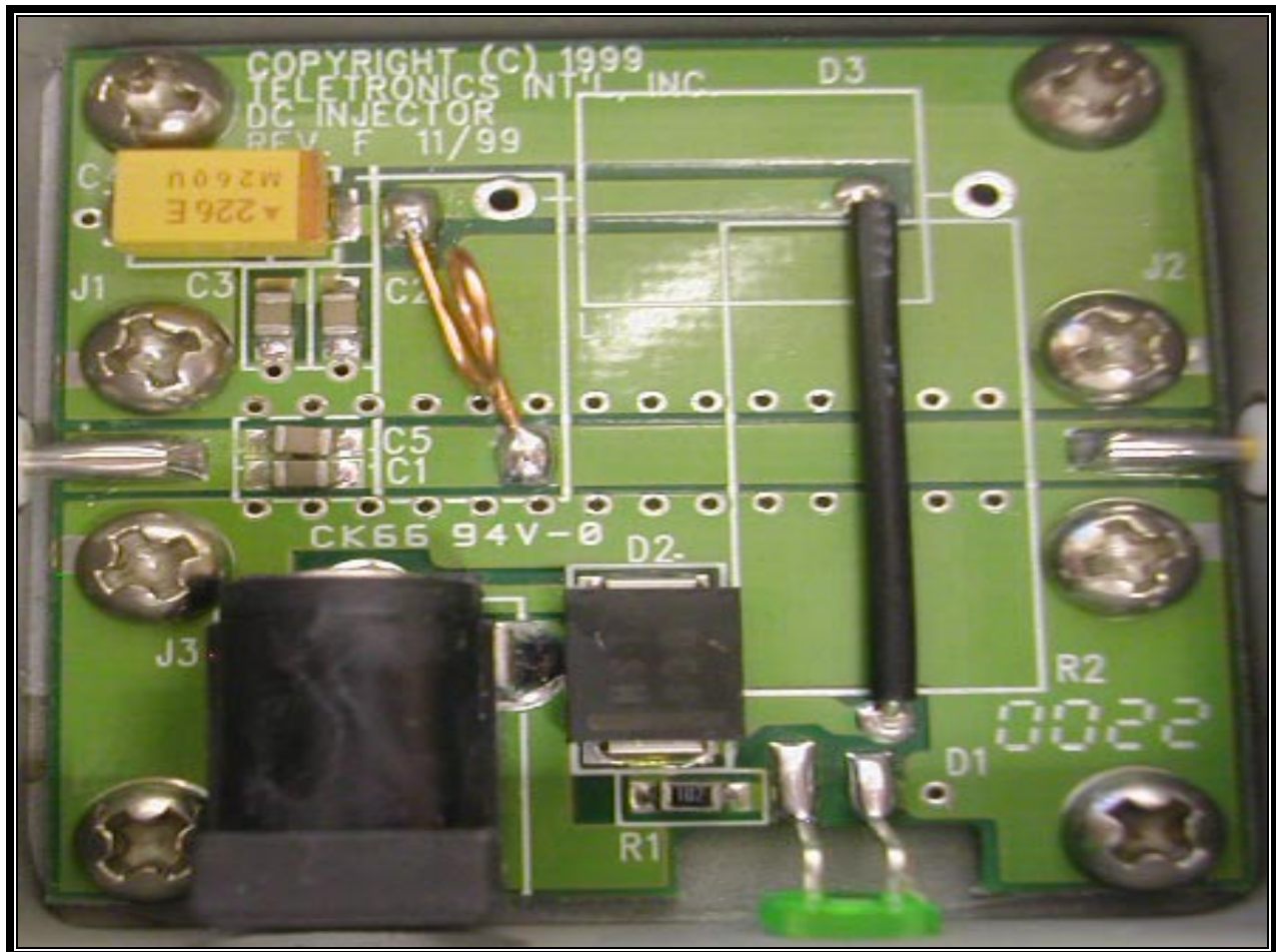
PHOTOGRAPH 23: FRONT VIEW PCB FROM DC INJECTOR
