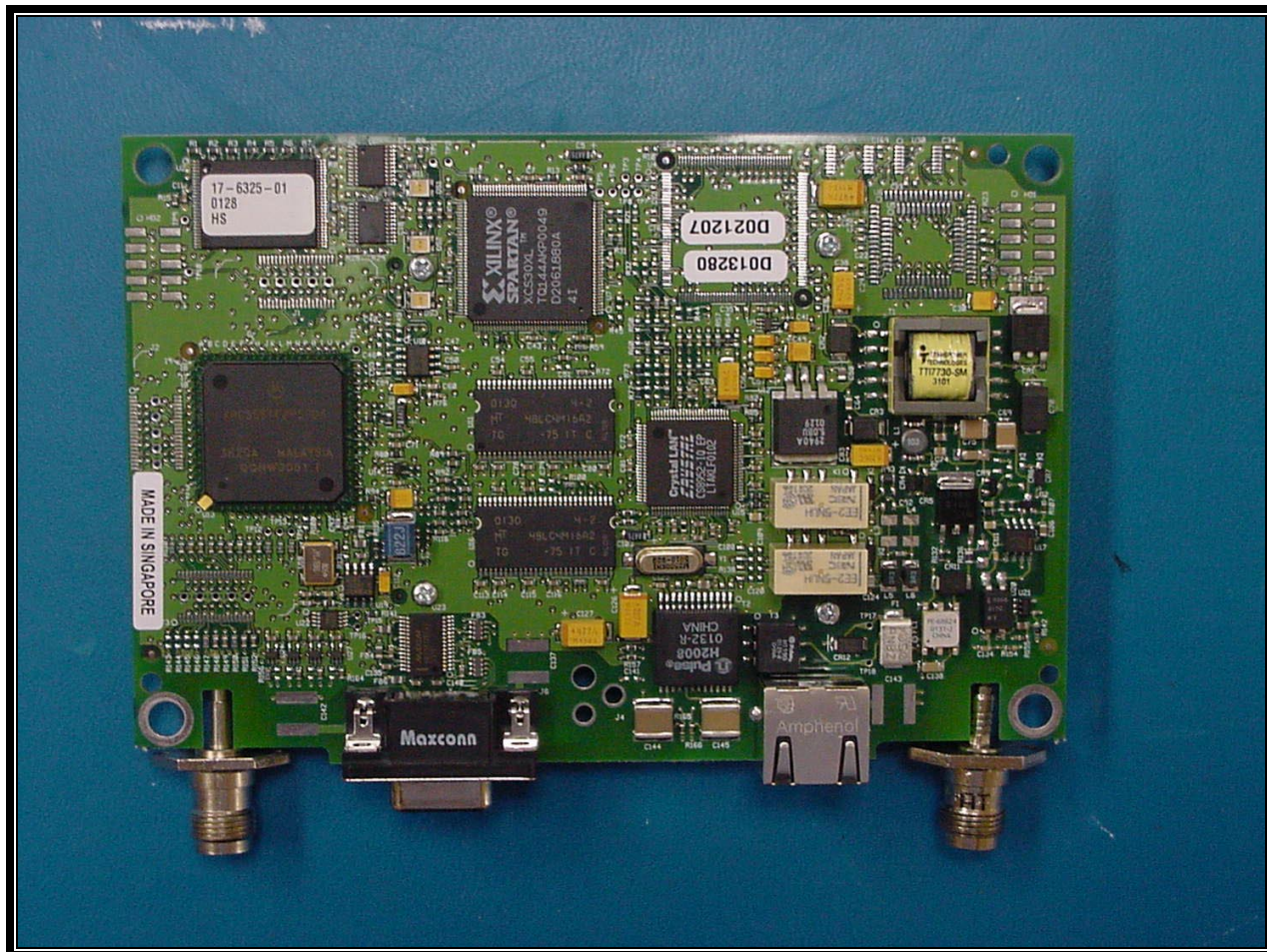
PHOTOGRAPH 22: FRONT VIEW DIGITAL PART OF THE ACCESS POINT
