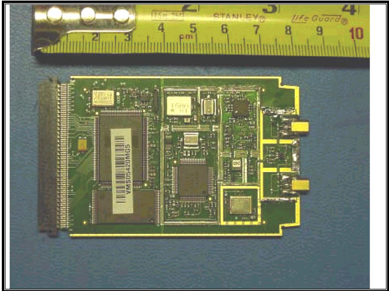
PHOTOGRAPH 19: BACK VIEW OF THE PCB WITHOUT SHIELD
