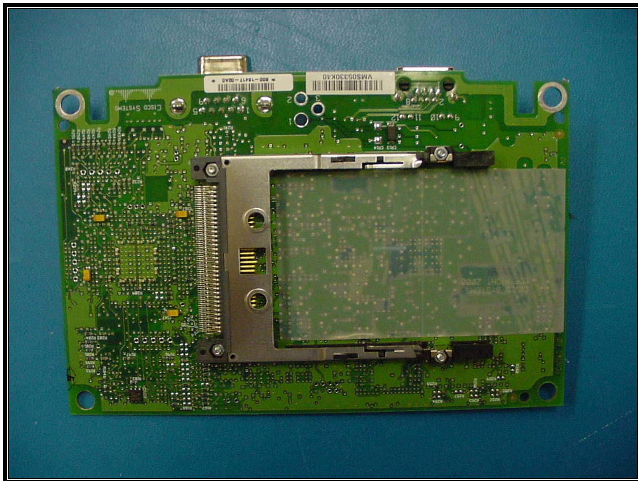
PHOTOGRAPH 21: FRONT VIEW DIGITAL PART OF THE ACCESS POINT
