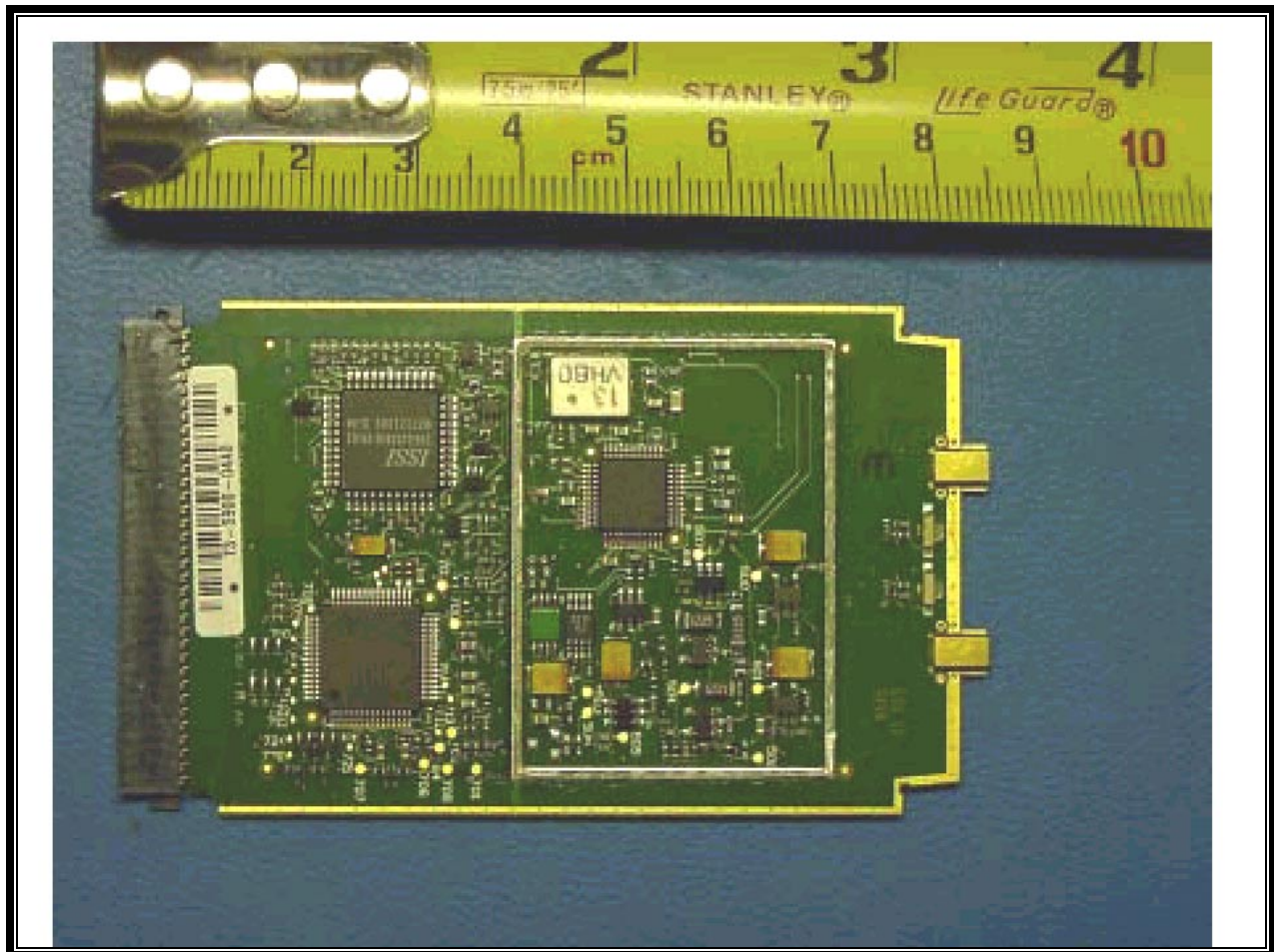
PHOTOGRAPH 17: FRONT VIEW OF PCB WITHOUT SHIELD
