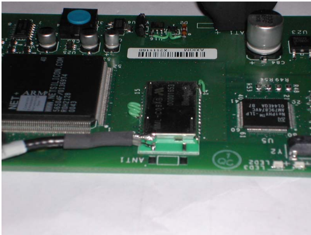
Old Main Board Antenna Term.
