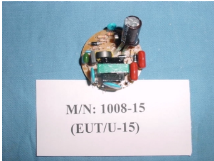
Figure 57 Main Board, Component Side
