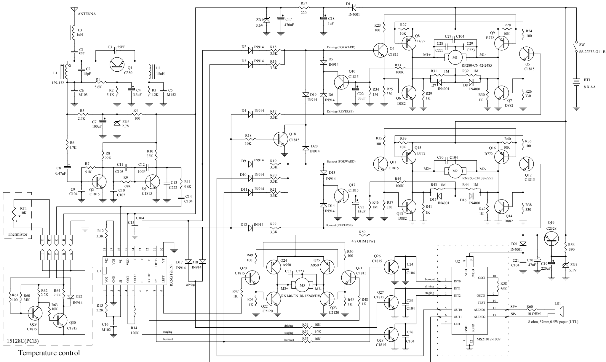
HERALD METAL & PLASTIC WORKS LTD. K'NEX #15128 (49MHZ) RECEIVER CIRCUIT DIAGRAM
