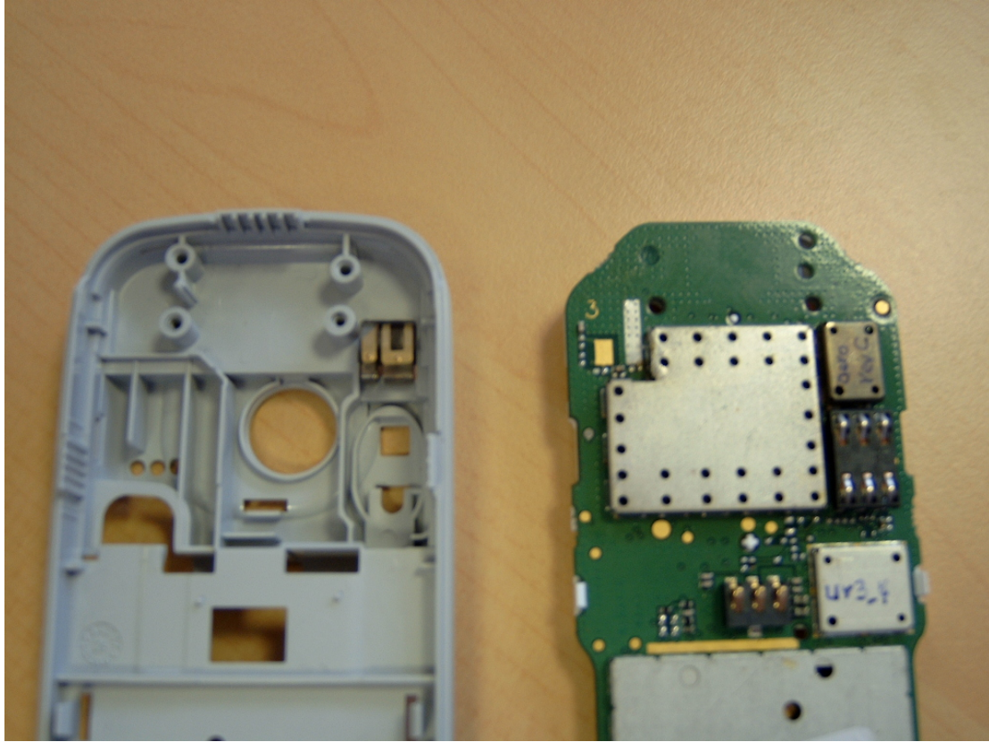
SND321 – Internal View- Antenna Connection Locations
