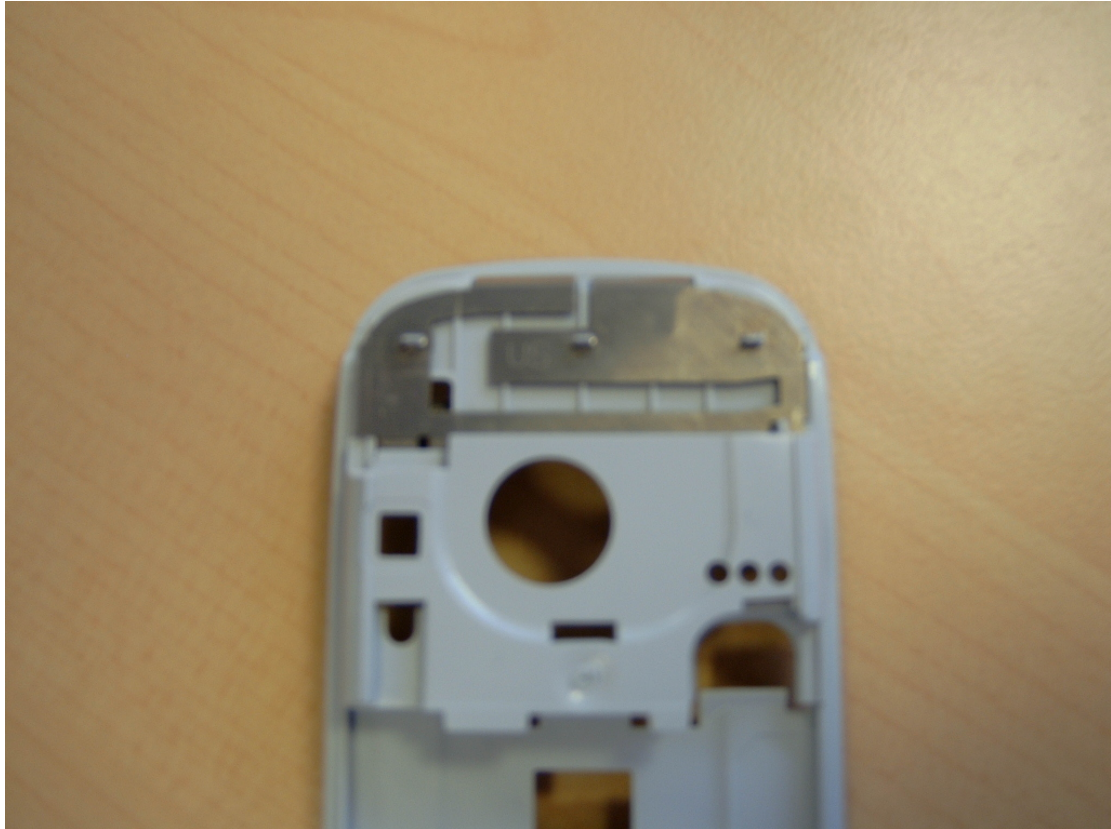
SND321 – Internal View - Antenna
