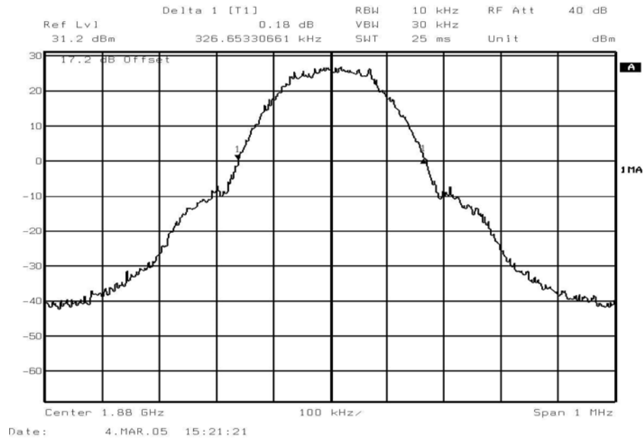
Maximum Power – Circuit Switched (GSM)
