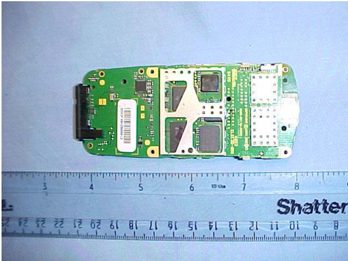
Main board bottom screening can top removed
