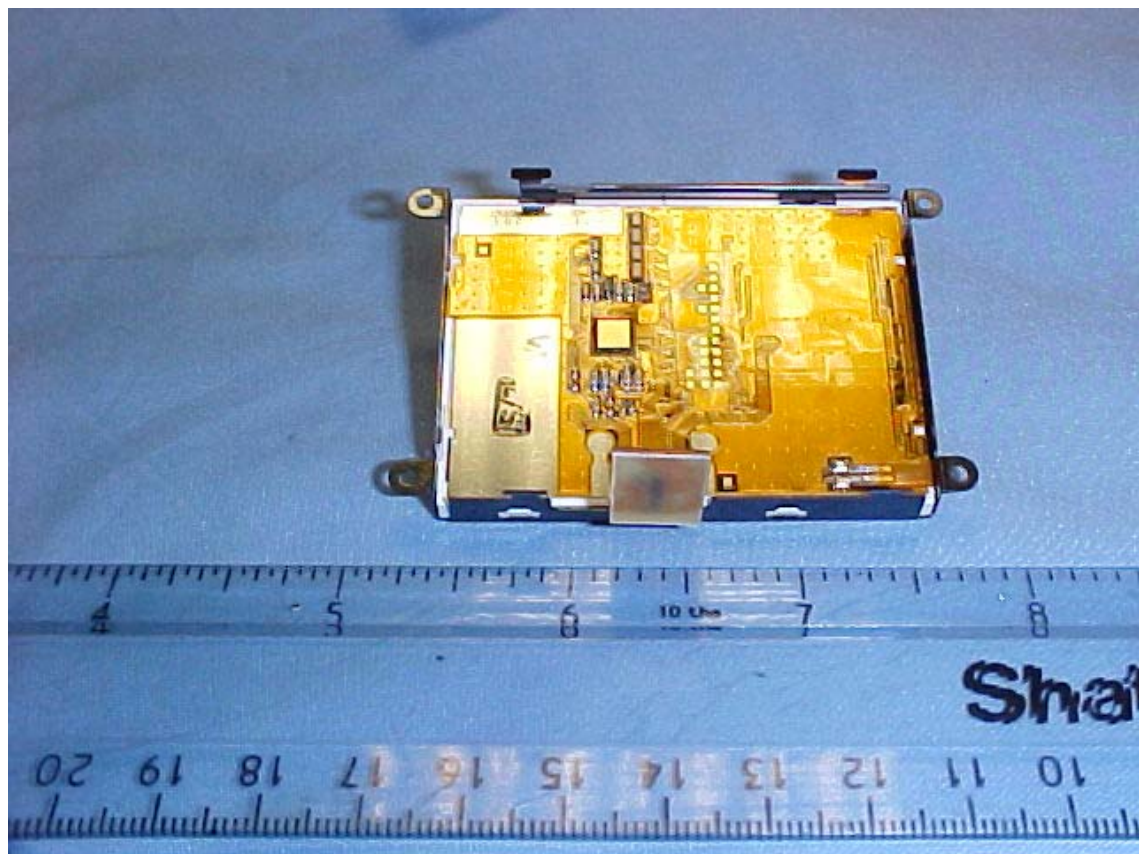
LCD display rear
