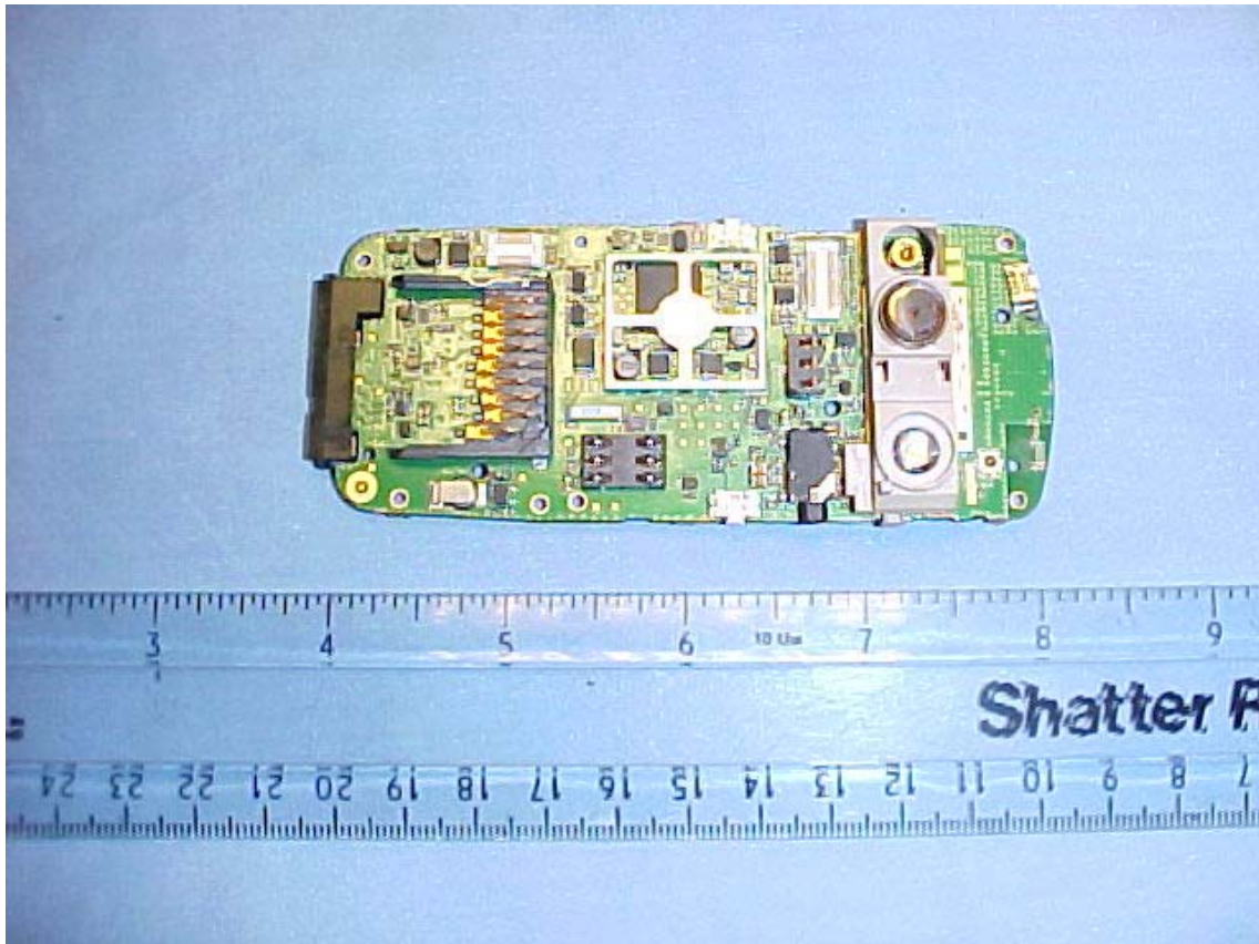
Main board top, screening can top removed
