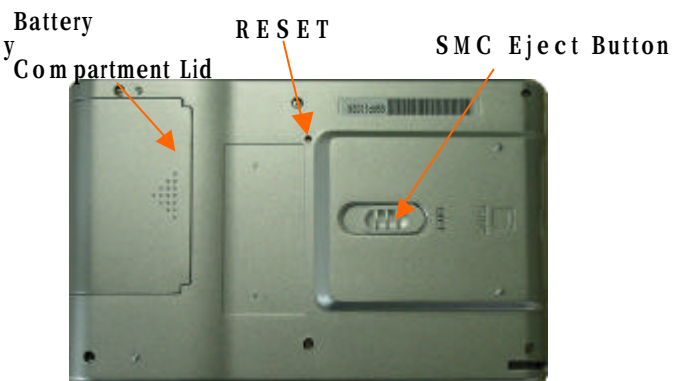
(2) Rear View
