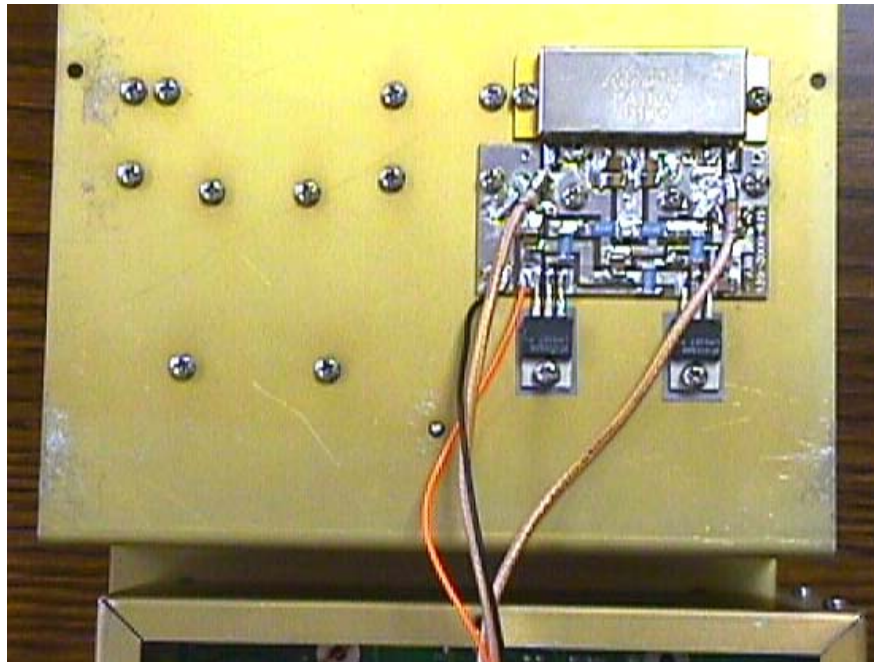
HEATSINK ASSEMBLY
