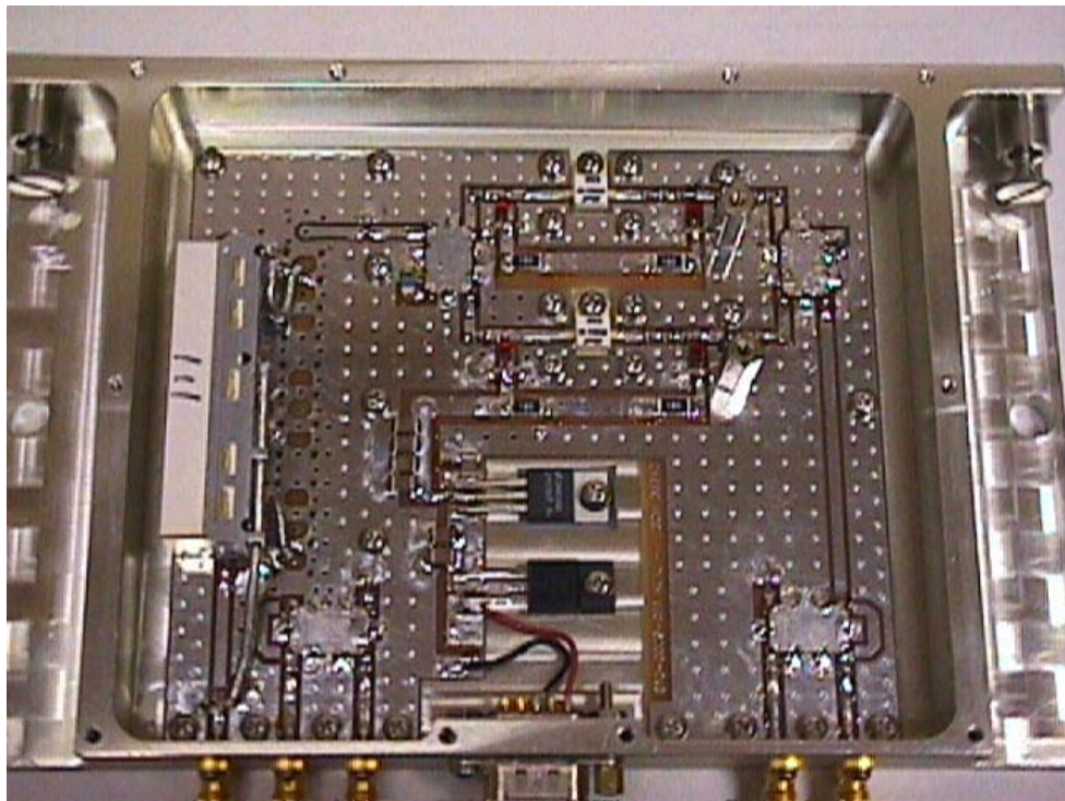
UPLINK/DOWNLINK AMPLIFIER MODULE
