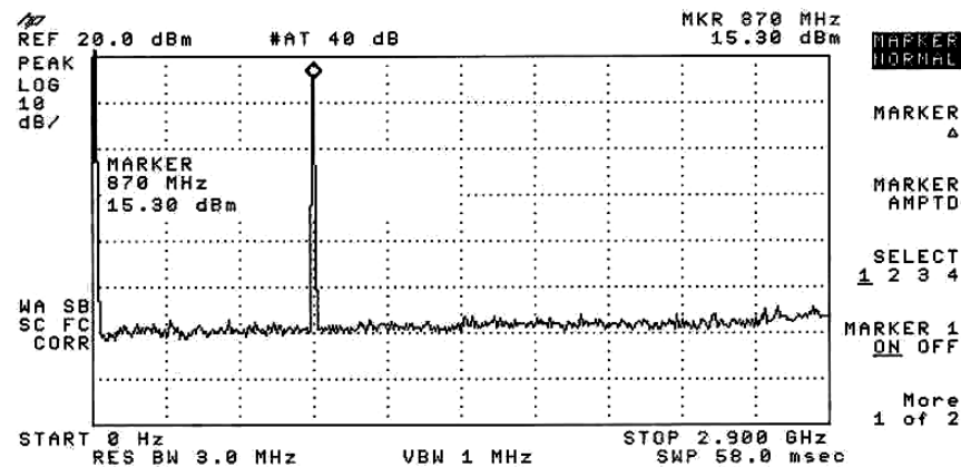
Plot 24 Antenna Terminal Emissions - SMR NADC Modulation
