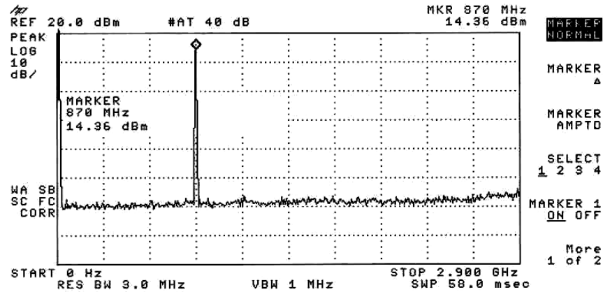
Plot 23 Antenna Terminal Emissions - SMR FM Modulation
