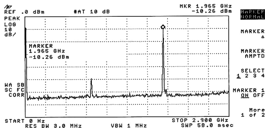
Plot 41 Radiated Spurious – PCS CDMA Modulation
