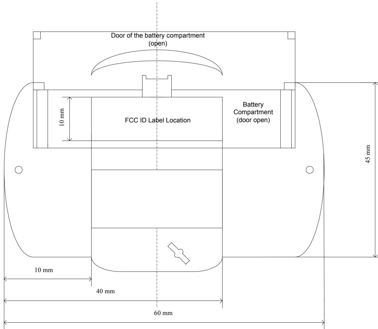
Location of the FCC ID Label in the Battery Compartment of the Base enclosure
