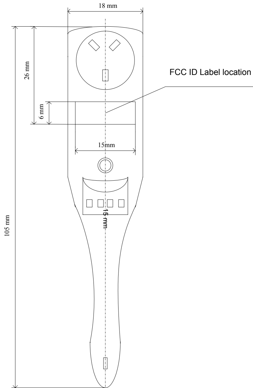
Headset Model : AD688H-X FCC ID label location on the front side of the enclosure
