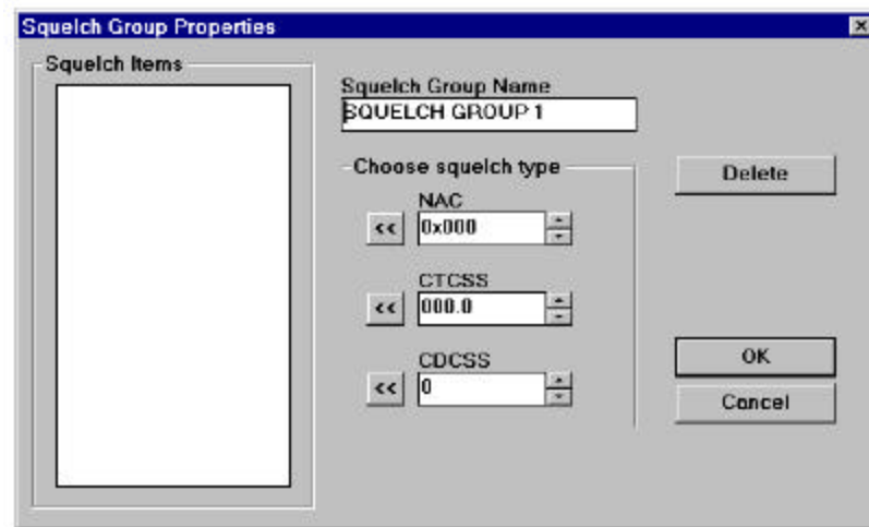
Figure 5-13 Squelch Groups Dialog Box
