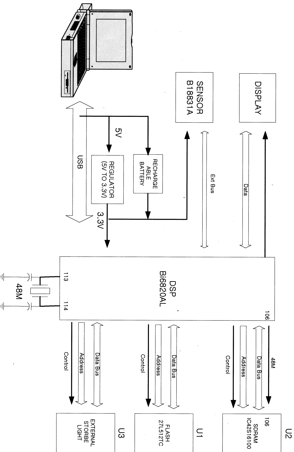
SP-130 Block Diagram
