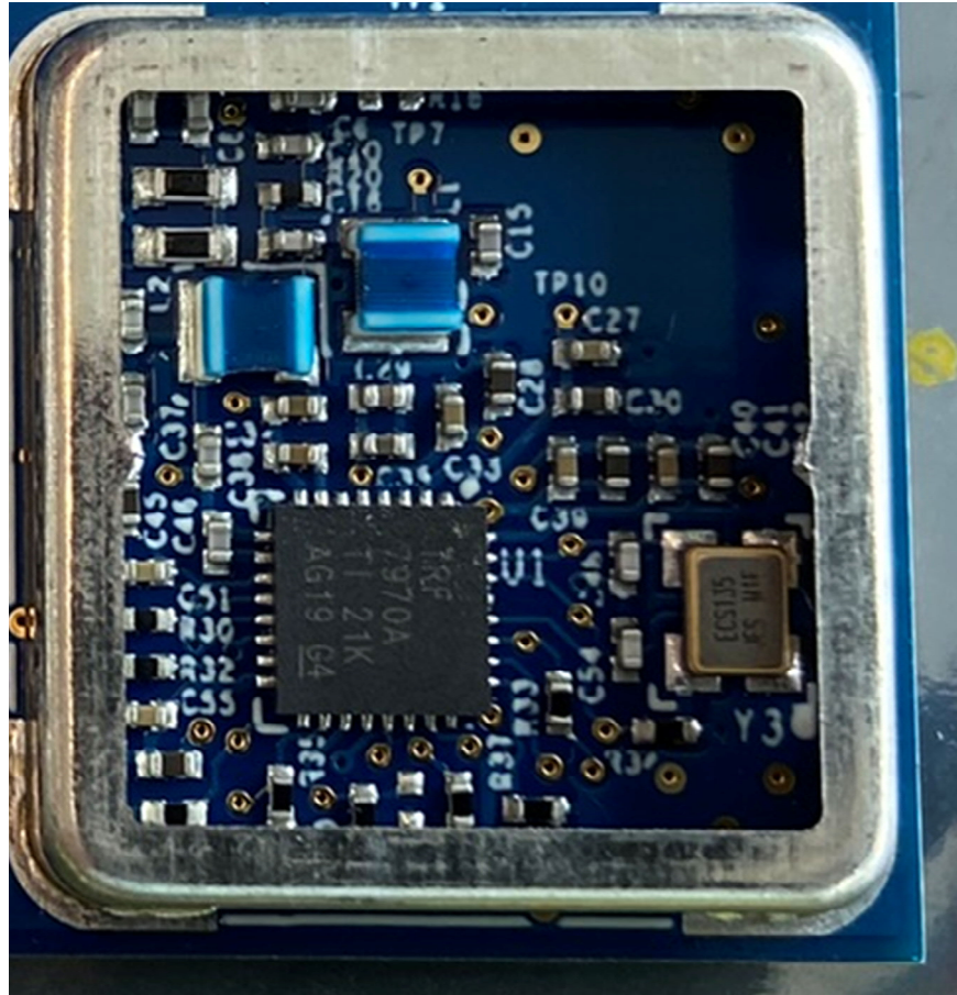
Figure 3: PT00121584 Secure RFID Reader Athena - RF IC location closeup
