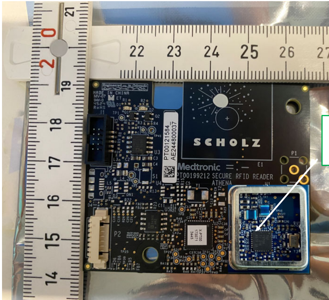
Figure 2: PT00121584 Secure RFID Reader Athena - Top View (RF IC location with shield removed)
