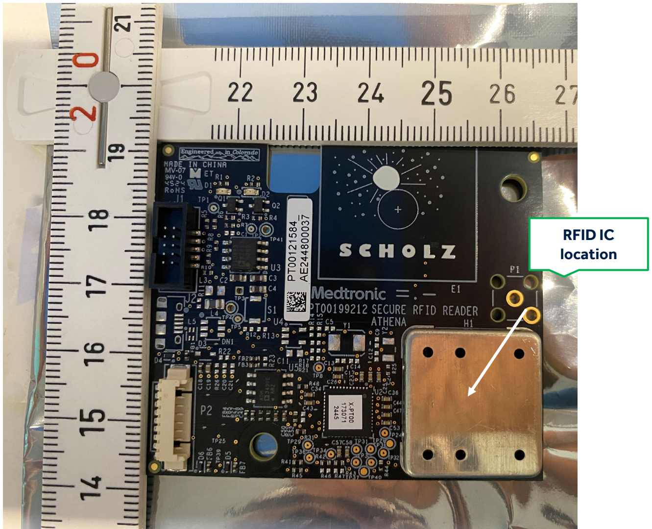
Figure 1: PT00121584 Secure RFID Reader Athena - Top View (RF IC location with shield)
