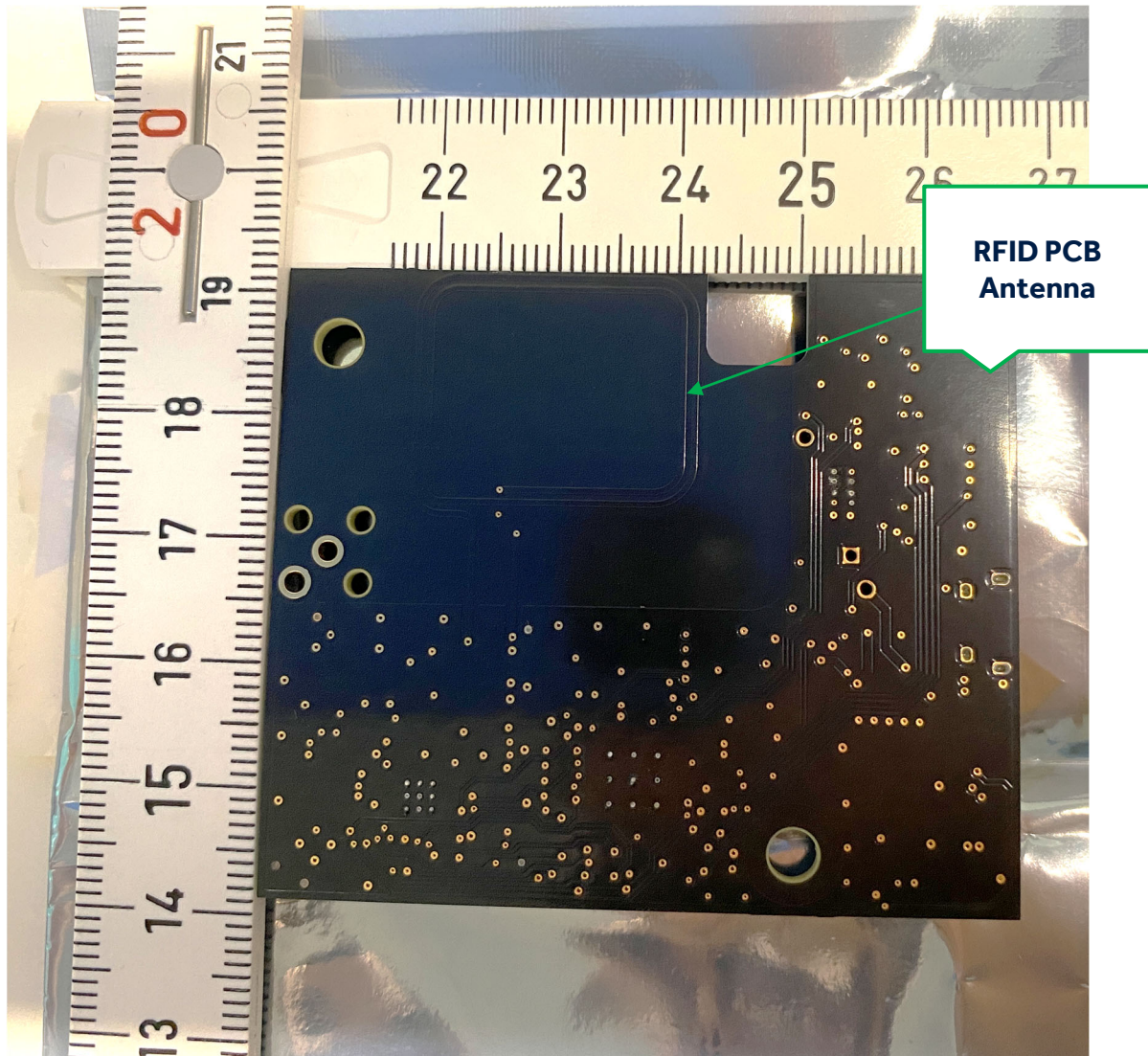
Figure 4: PT00121584 Secure RFID Reader Athena - Bottom View (antenna location)
