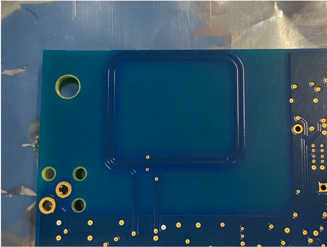
Figure 5: PT00121584 Secure RFID Reader Athena - Antenna closeup
