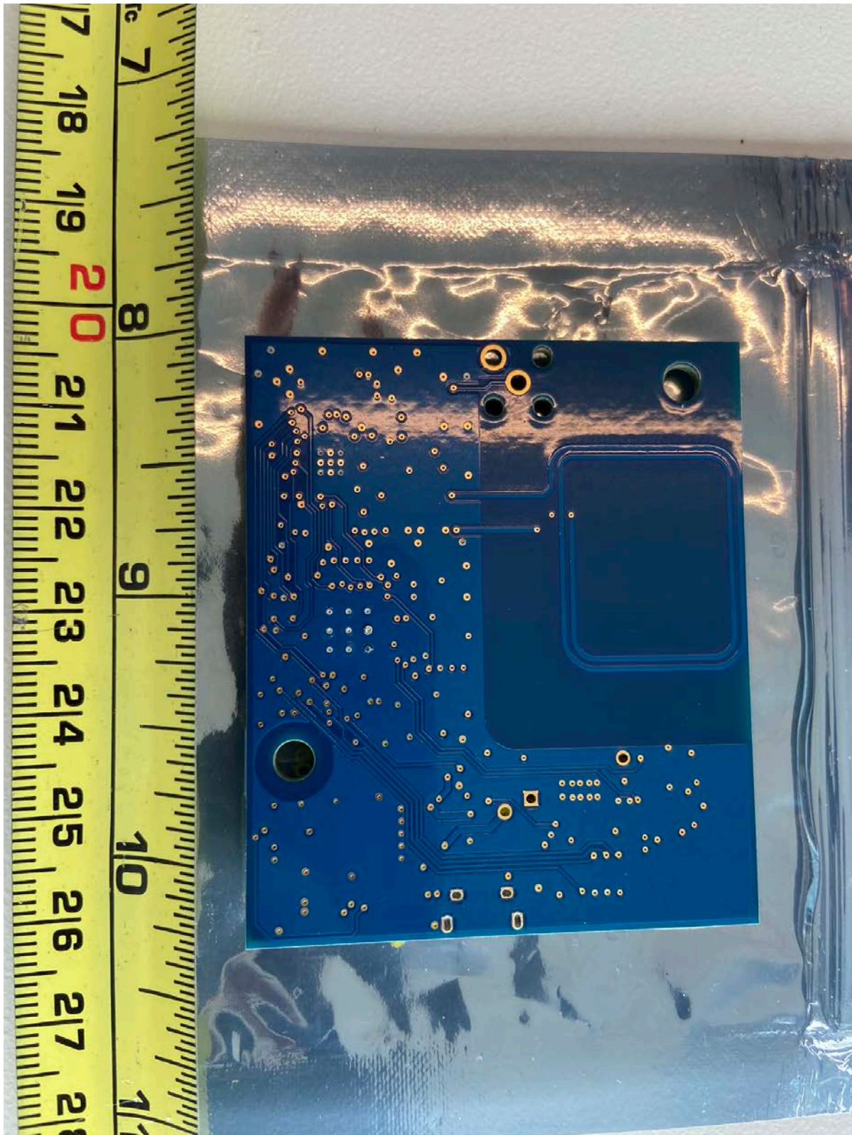
Figure 4: Module PCBA bottom view
