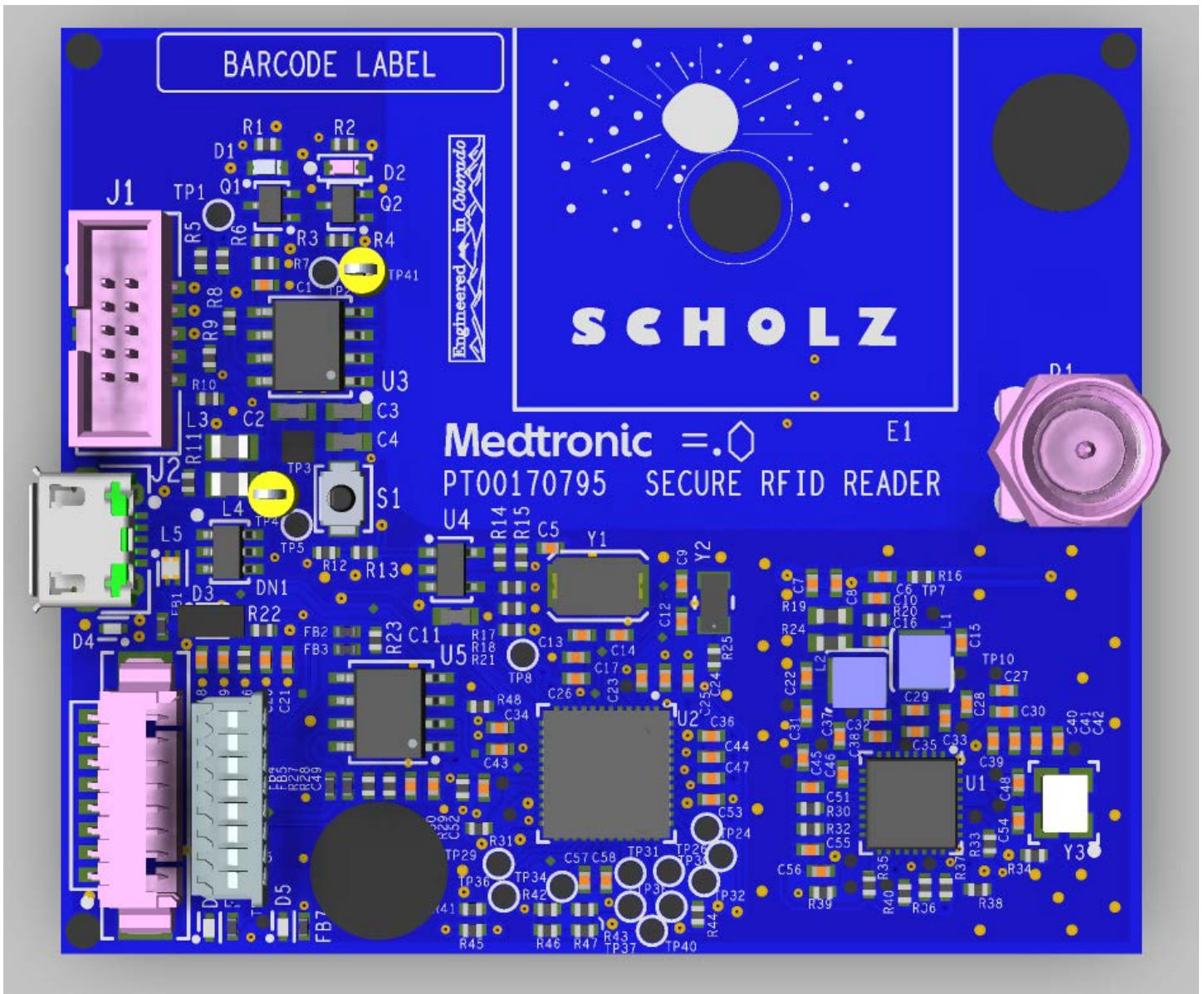
Figure 3: Module Top view PCBA-3D
