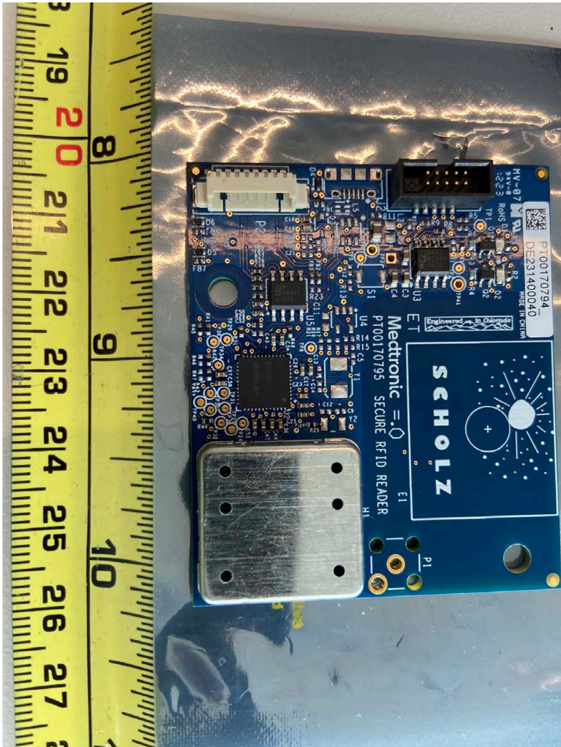
Figure 1: Module PCBA top view
