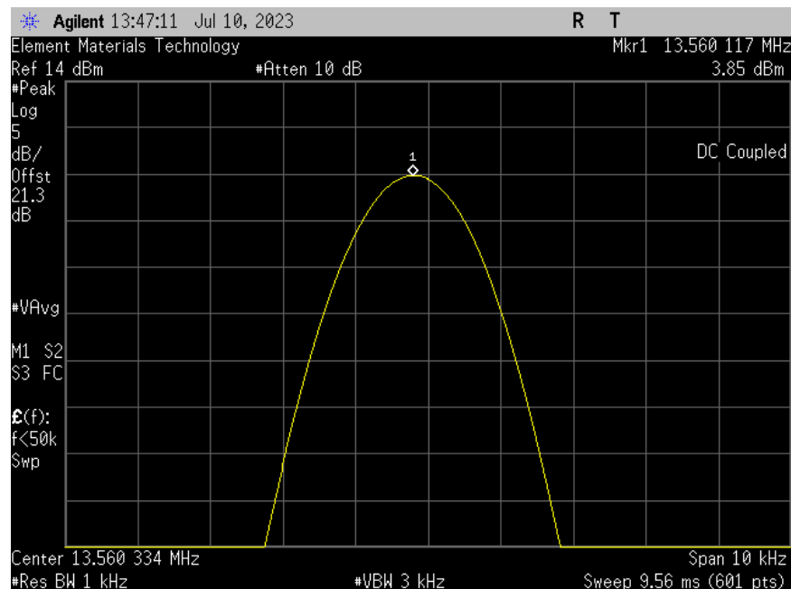
13.56 MHz RFID; Extreme Temperature +0°C
