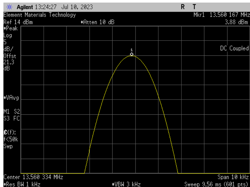
13.56 MHz RFID; Extreme Temperature +10°C
