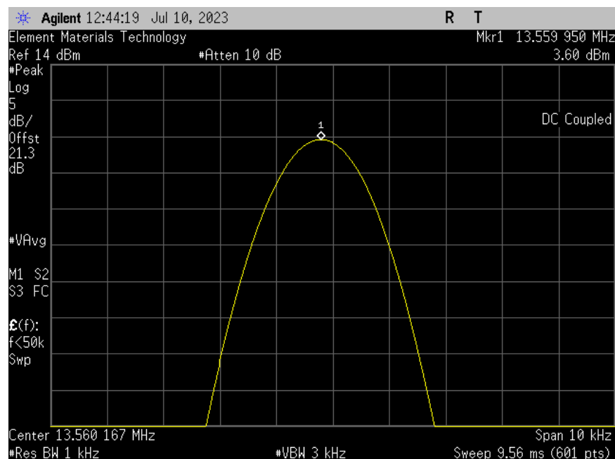
13.56 MHz RFID; Extreme Temperature +20°C
