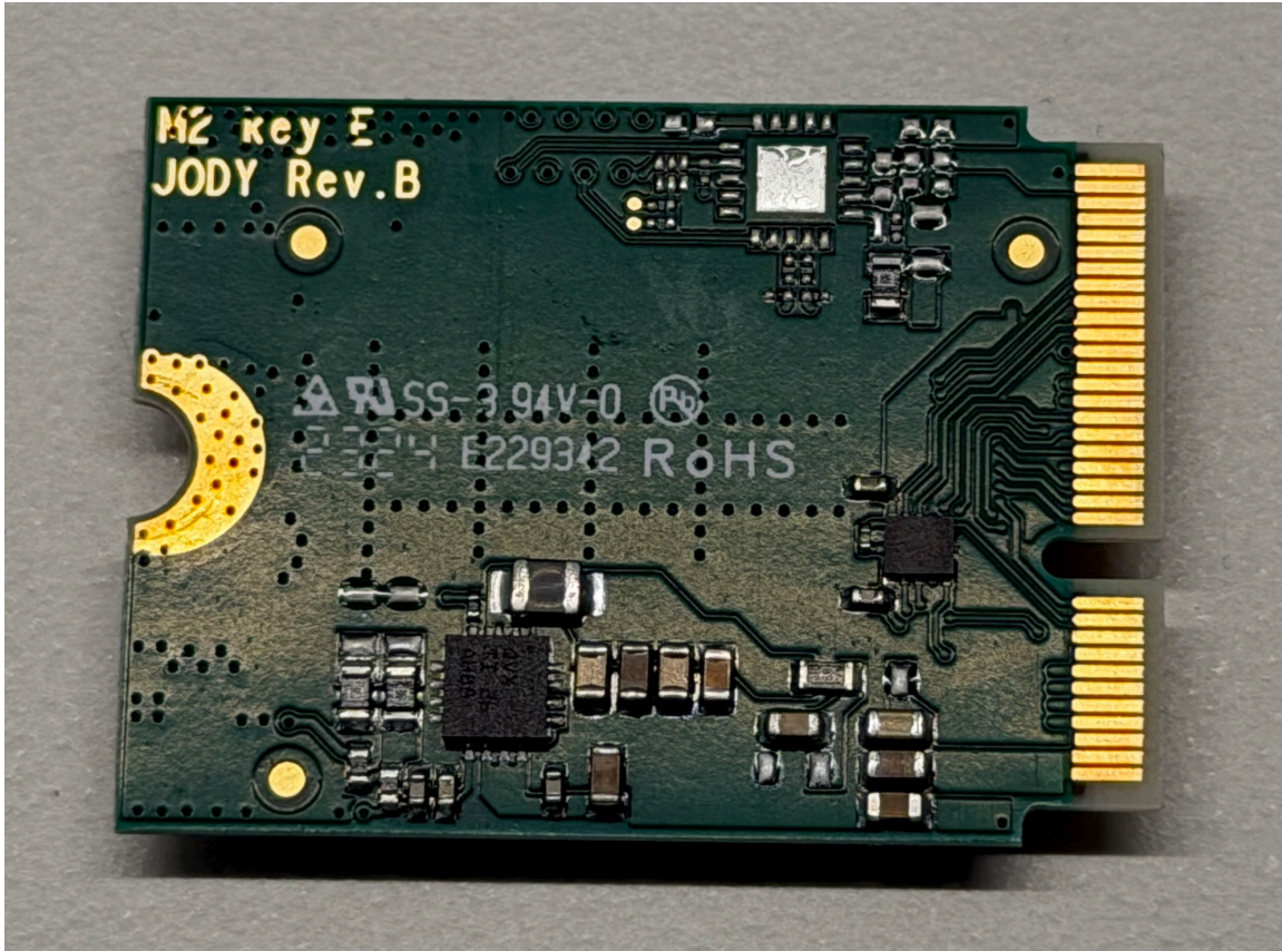
Figure 2: Radio module close-up photo -Bottom View
