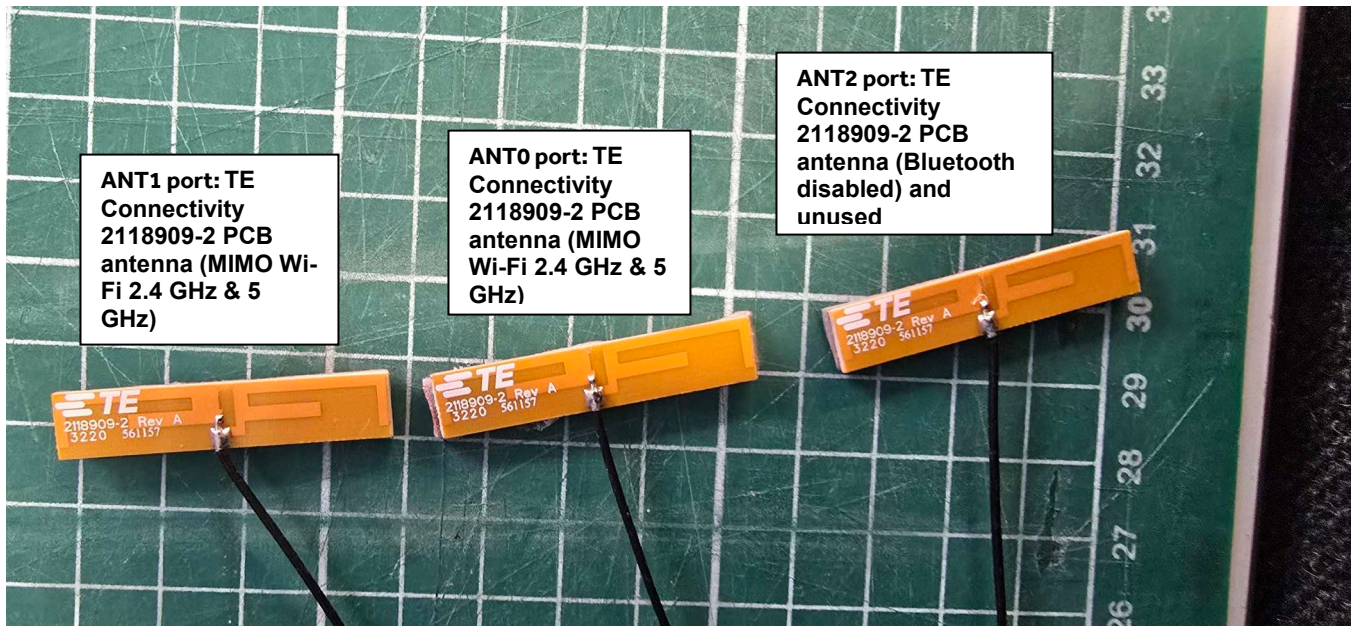
Figure 5: Three Identical Antennas TE Connectivity 2118909-2 Close-up View
