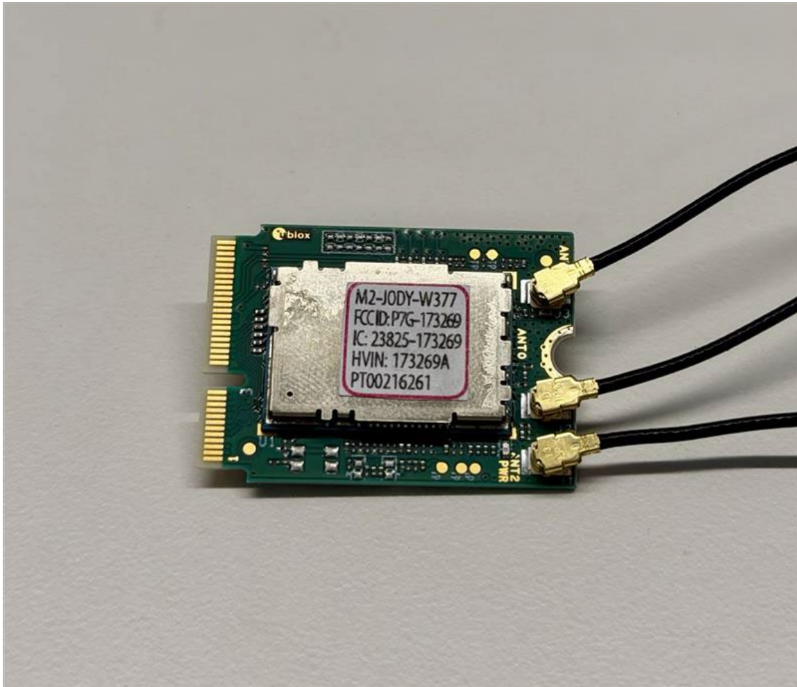
Figure 2: Radio module close-up photo - Top View
