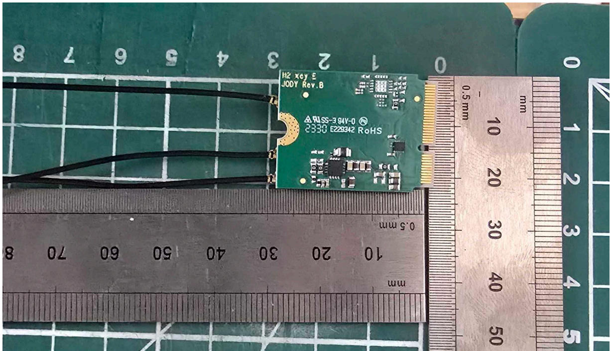
Figure 3: Radio module close-up photo -Bottom View
