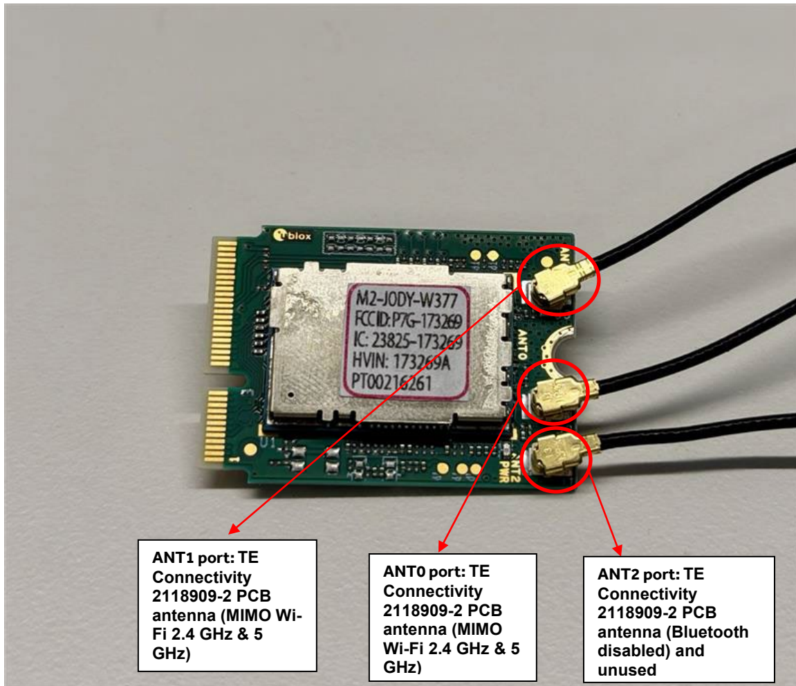
Figure 4: Radio module antenna ports
