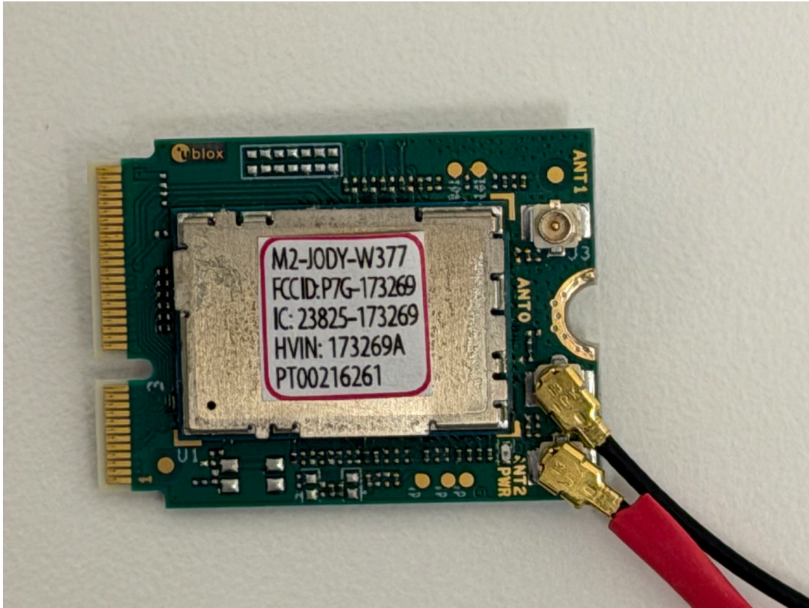
Figure 2: Radio module close-up with label
