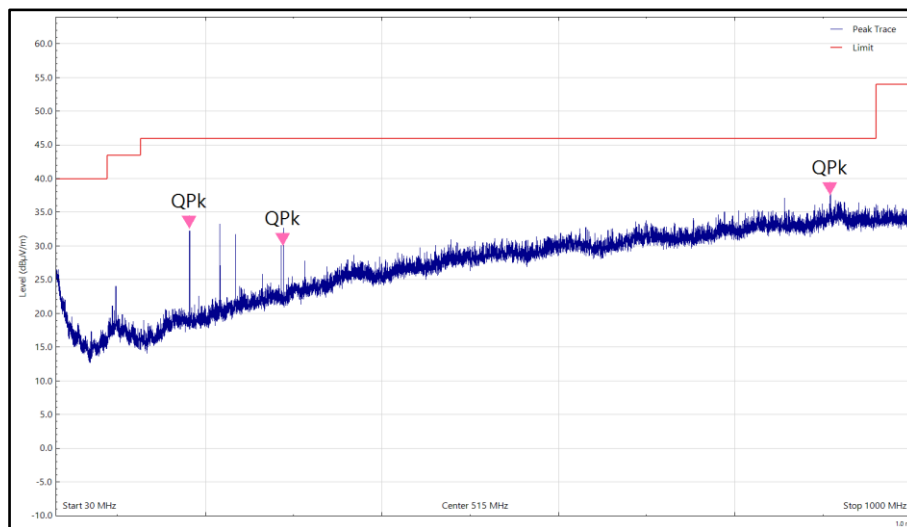
RSE, 30MHz-1GHz, 30 MHz to 1 GHz, Horizontal
