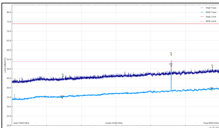
RSE, 5 to 8 GHz, 5 GHz to 8 GHz, Vertical
