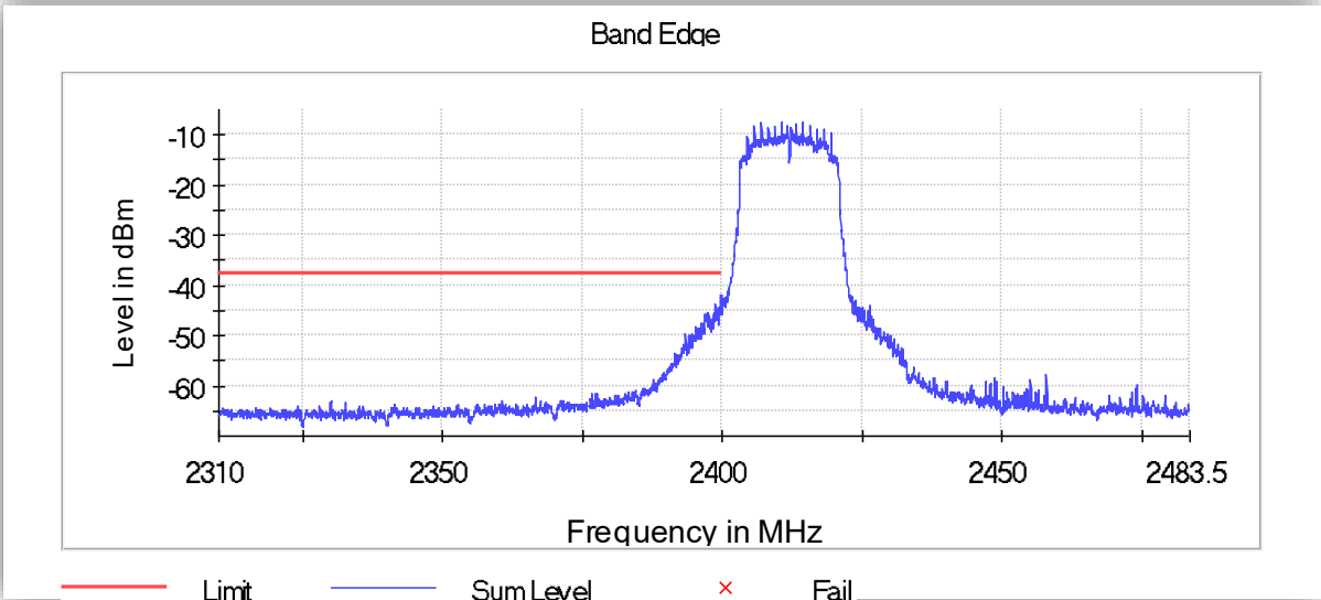
WLAN 802.11n MCS0 Low Band Edge 2400MHz
