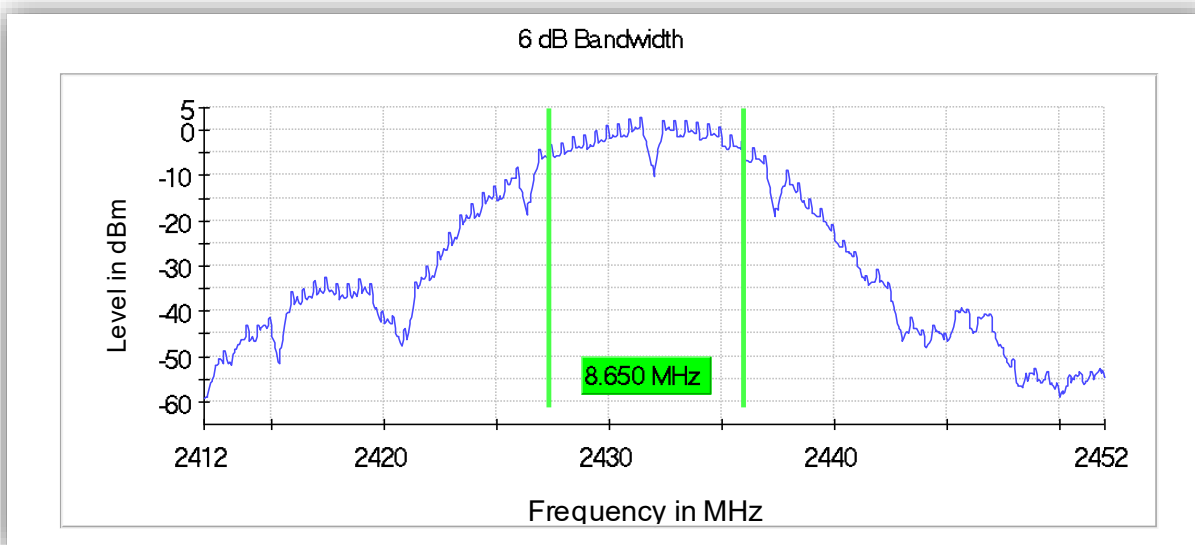
WLAN 802.11b 1Mbps Middle Channel
