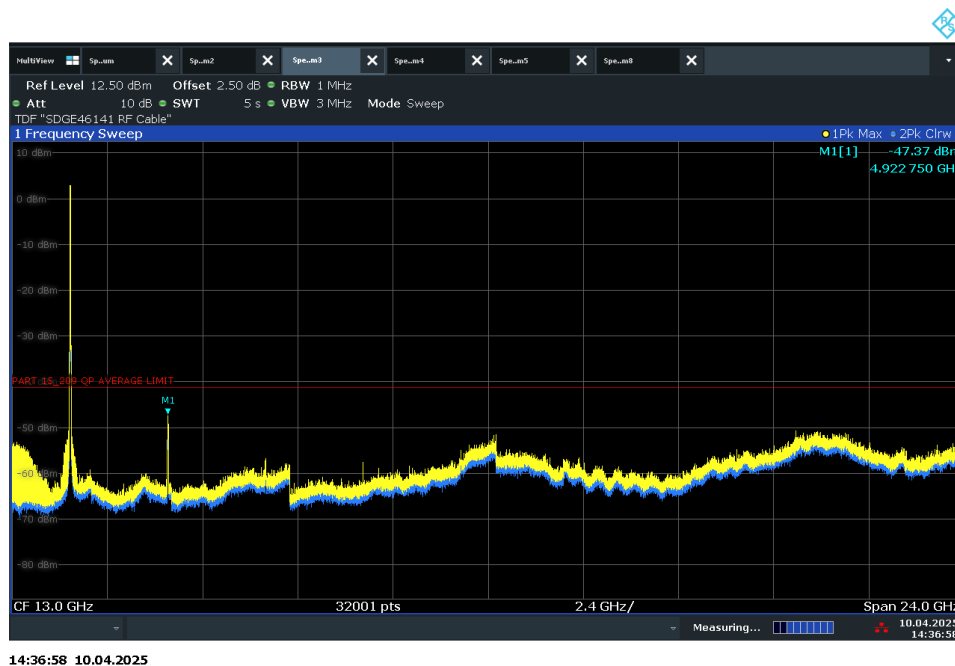
WLAN 802.11n MCS0 High Channel (1GHz to 25GHz)
