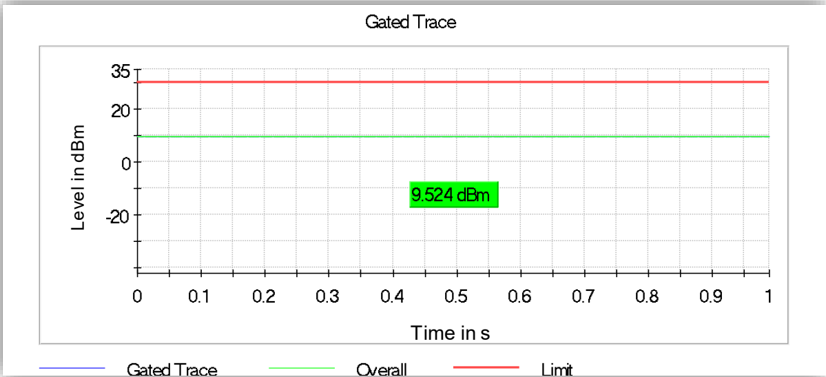
WLAN 802.11n MCS0 Mid Channel
