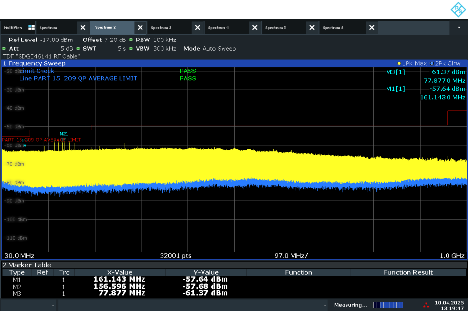
WLAN 802.11g 6Mbps Mid Channel (30MHz to 1GHz)
