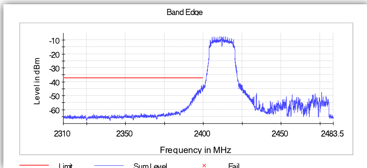
WLAN 802.11g 6Mbps Low Band Edge 2400MHz
