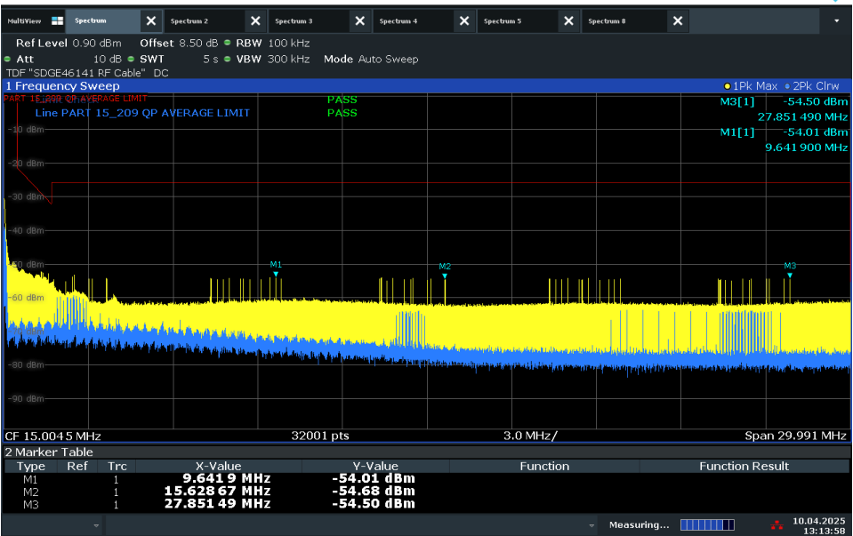
WLAN 802.11g 6Mbps Mid Channel (9kHz to 30MHz)
