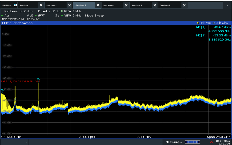
WLAN 802.11b 1Mbps High Channel (1GHz to 25GHz)
