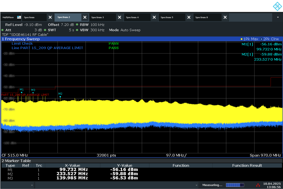
WLAN 802.11g 6Mbps Low Channel (30MHz to 1GHz)
