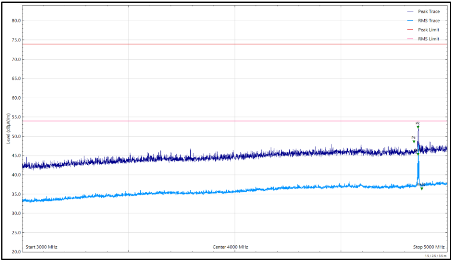
RSE, 1 to 5 GHz, 3 GHz to 5 GHz, Vertical
