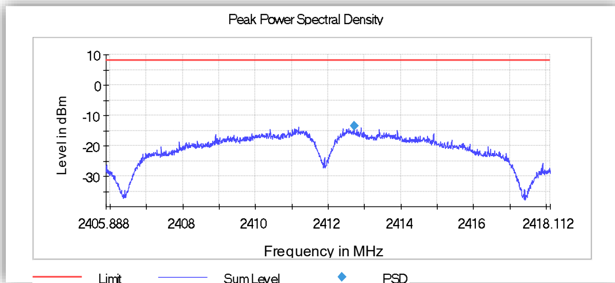
WLAN 802.11b 1Mbps Low Channel
