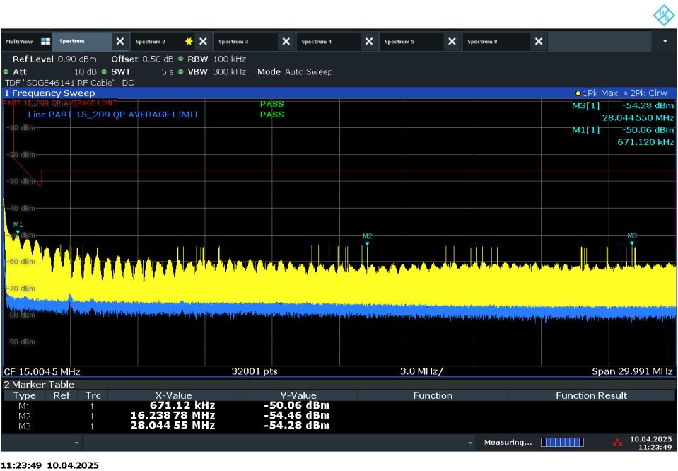
WLAN 802.11b 1Mbps Low Channel (9kHz to 30MHz)
