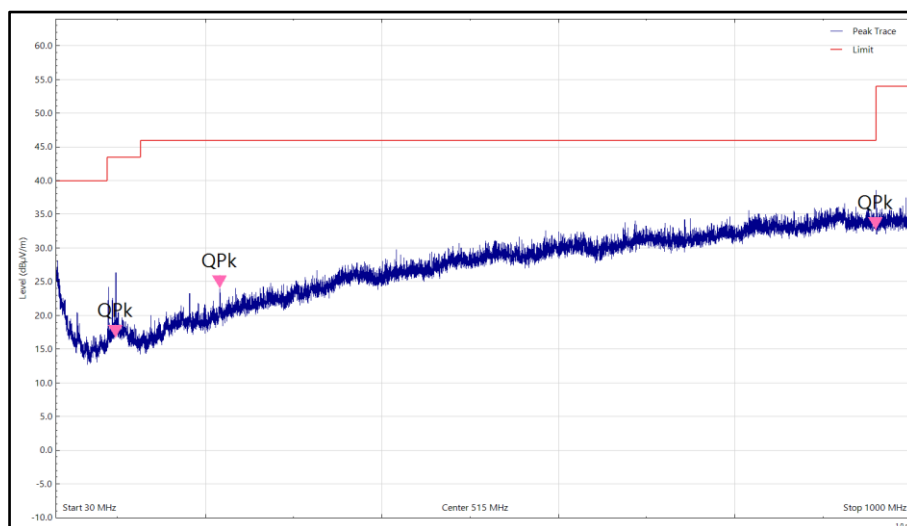
RSE, 30MHz-1GHz, 30 MHz to 1 GHz, Vertical
