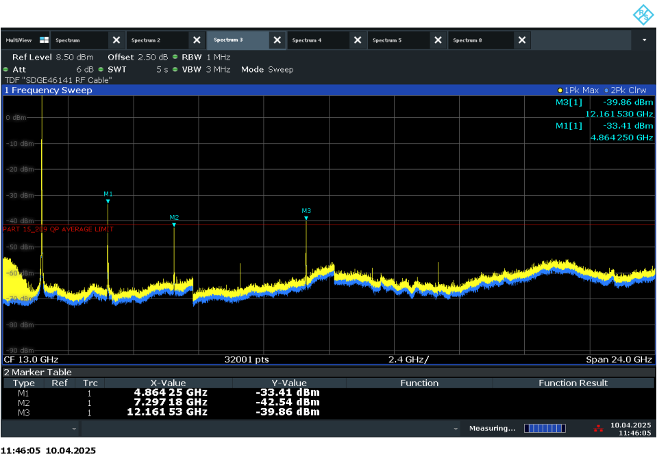
WLAN 802.11b 1Mbps Mid Channel (1GHz to 25GHz)
