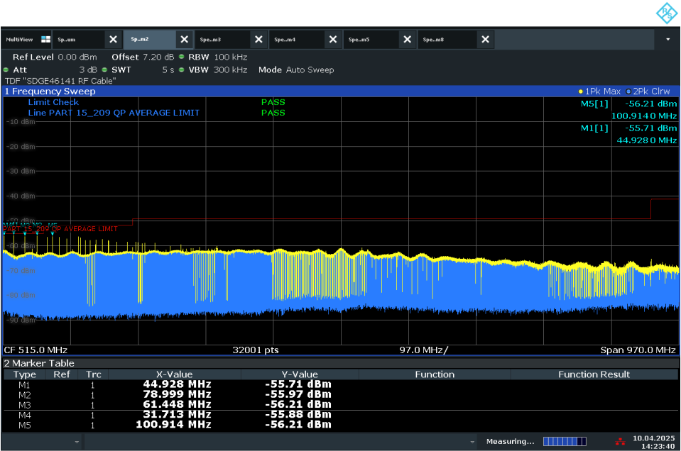
WLAN 802.11n MCS0 Mid Channel (30MHz to 1GHz)
