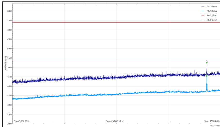
RSE, 1 to 5 GHz, 3 GHz to 5 GHz, Horizontal
