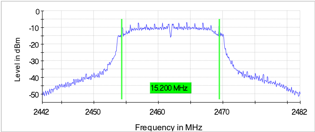
6 dB Bandwidth
