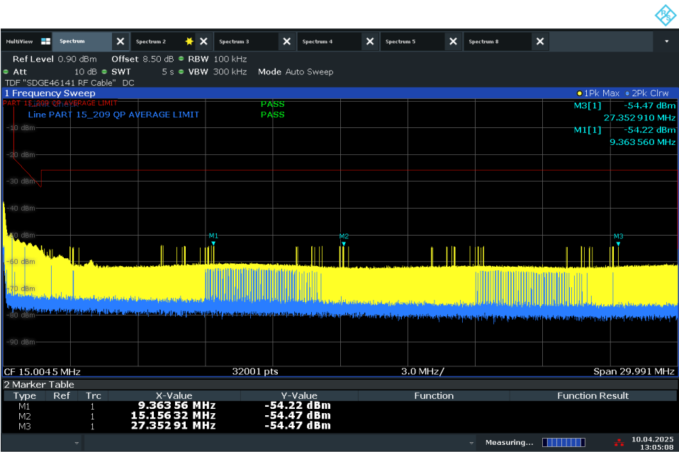
WLAN 802.11g 6Mbps Low Channel (9kHz to 30MHz)
