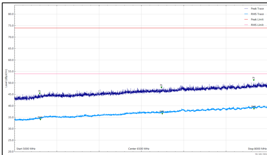
RSE, 5 to 8 GHz, 5 GHz to 8 GHz, Horizontal
