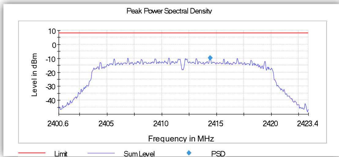
WLAN 802.11g 6Mbps Low Channel
