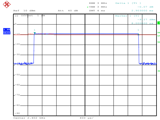
Figure 8. Plot of the Time of Occupancy (Conducted)
