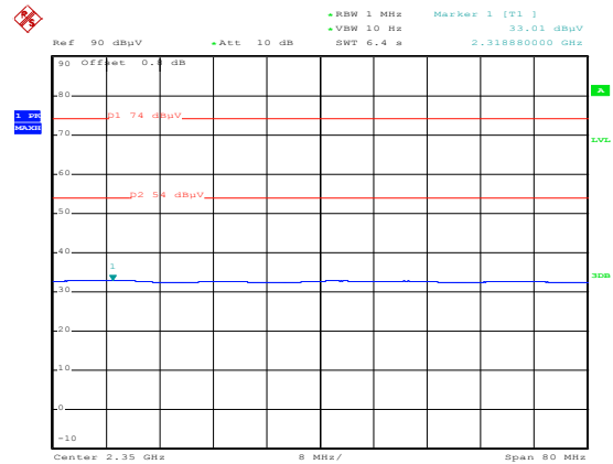
Lowest Channel(2 402 MHz): AVERAGE
