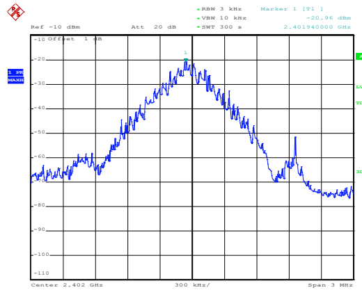
Figure 16. Plot of the Peak Power Spectral Density (Conducted) - GFSK
