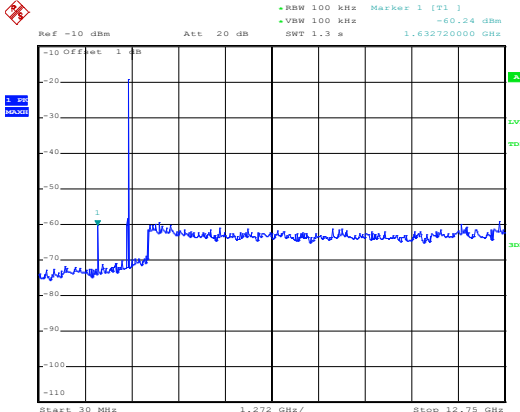
Highest Channel(2 480 MHz):30MHz~12.75GHz
