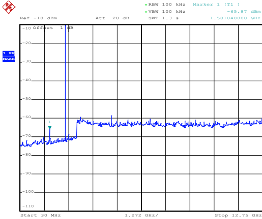
Figure 12. Plot of the Spurious RF conducted emissions - GFSK
