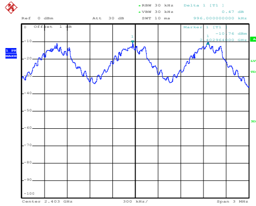
Figure 3. Plot of the Carrier Frequency Separation (Conducted)
