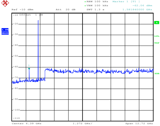
Lowest Channel(2 402 MHz):30MHz~12.75GHz
