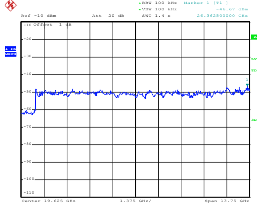
Middle Channel(2 440 MHz):12.75~26.5GHz
