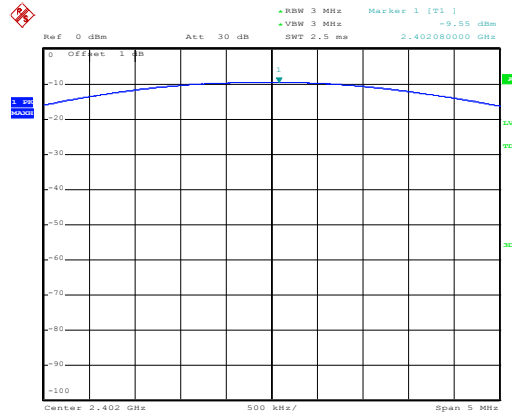
Figure 1. Plot of the Maximum Peak Output Power (Conducted) - GFSK
