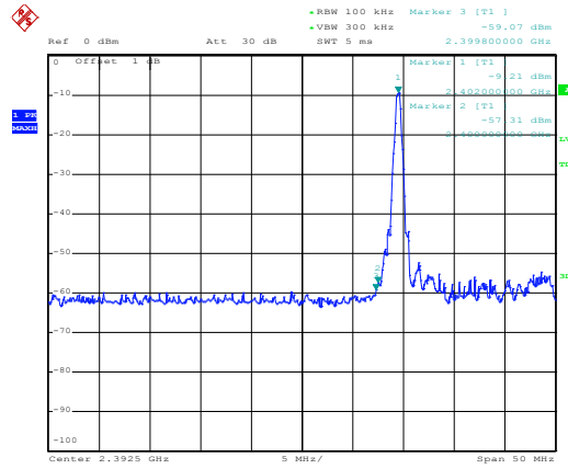
Figure 10. Plot of the Band Edge (Conducted)
