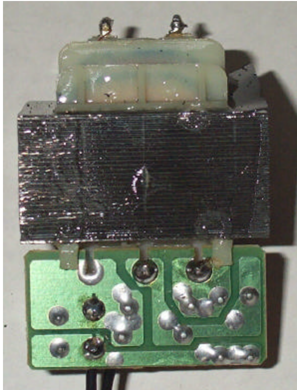
Transformer Foil Side
