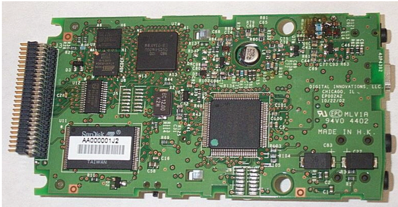
Processor and RF PCB
