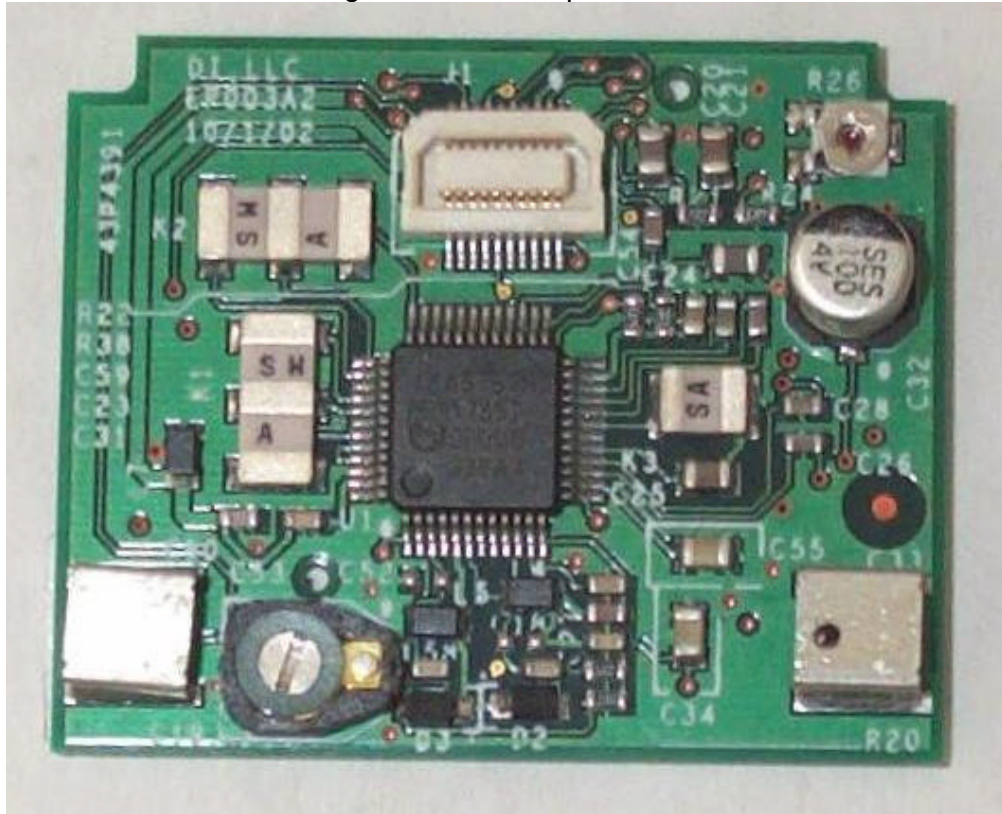
Daughter Board Component Side
