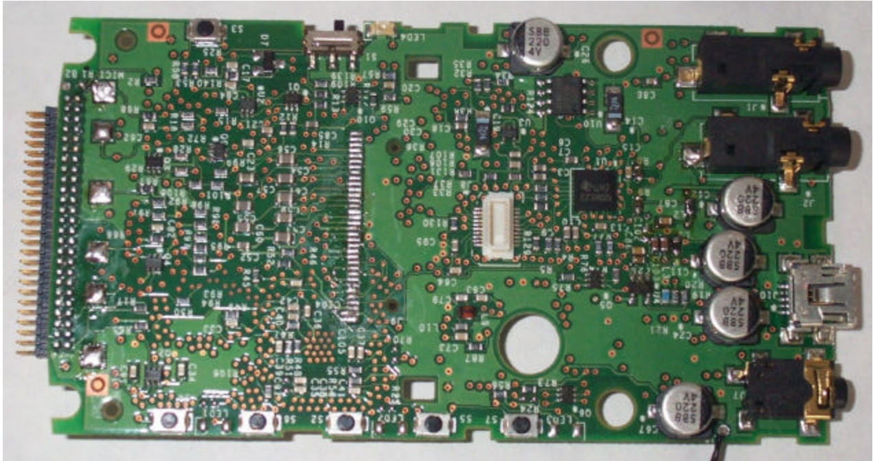
Processor and RF PCB
