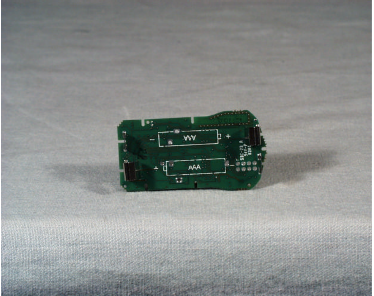
Bottom view of the SLFPR100 PCB (Remote)
