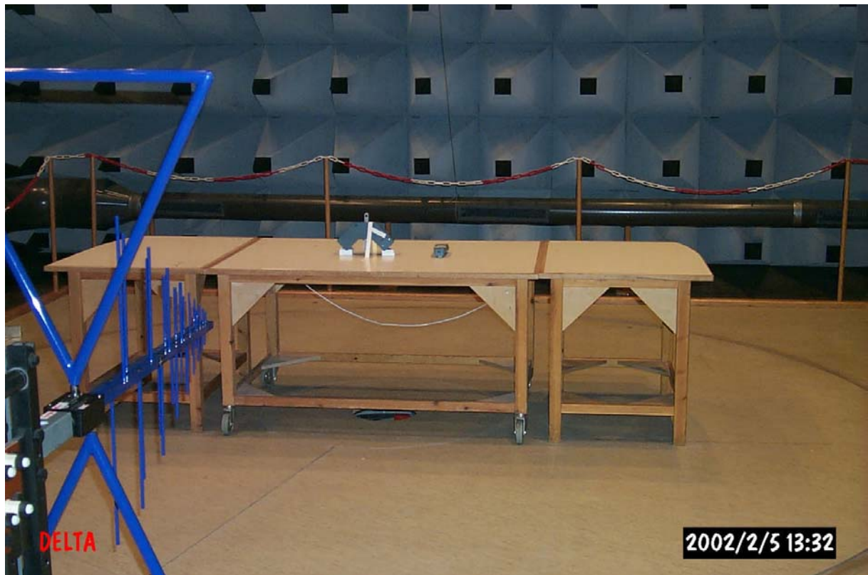
Photo 1 Set-up for measurements 30 MHz to 1000 MHz. EUT to the left. A transceiver from the same product family is monitored in receive only mode.
