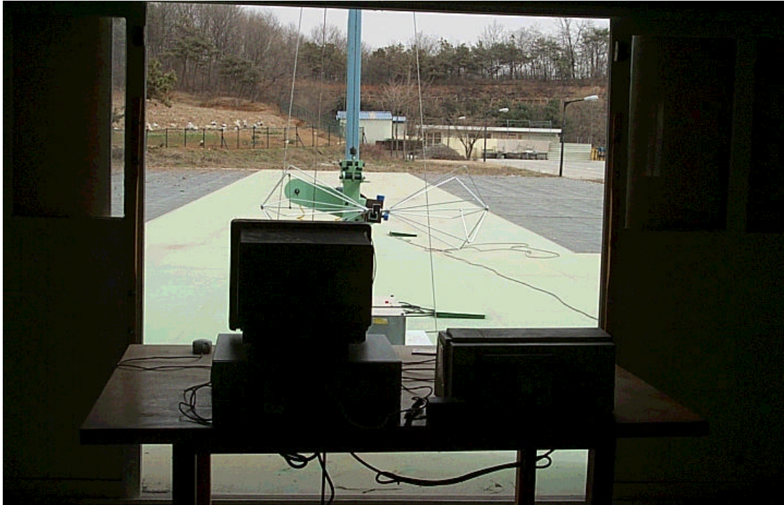
Photograph 2 : Setup for Radiated Emissions
