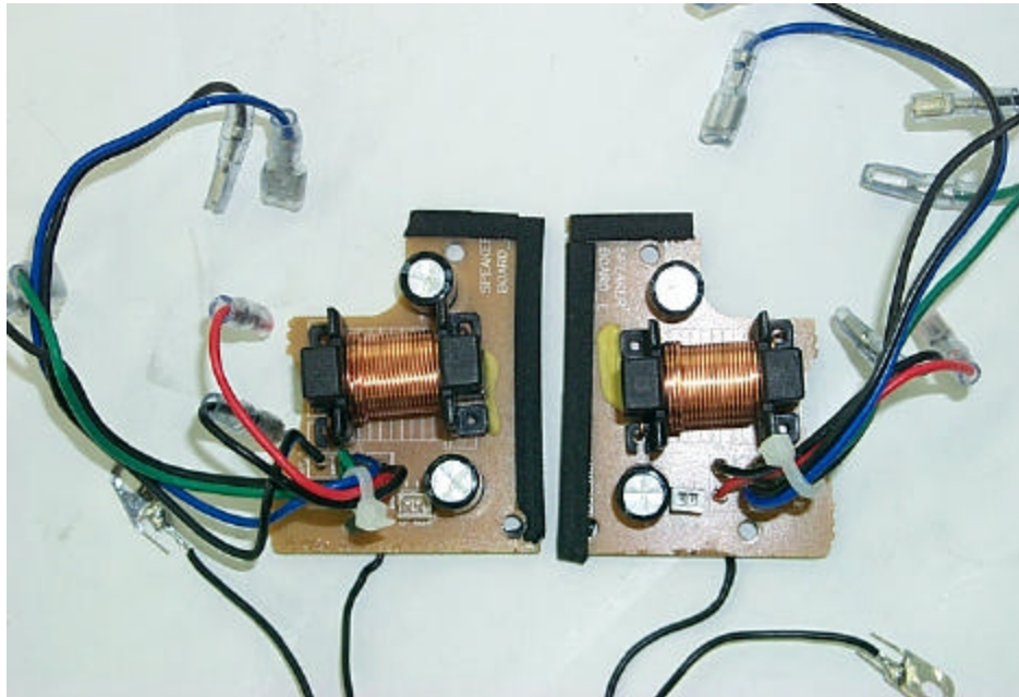
< Speaker Board(L/R) – Top View >
