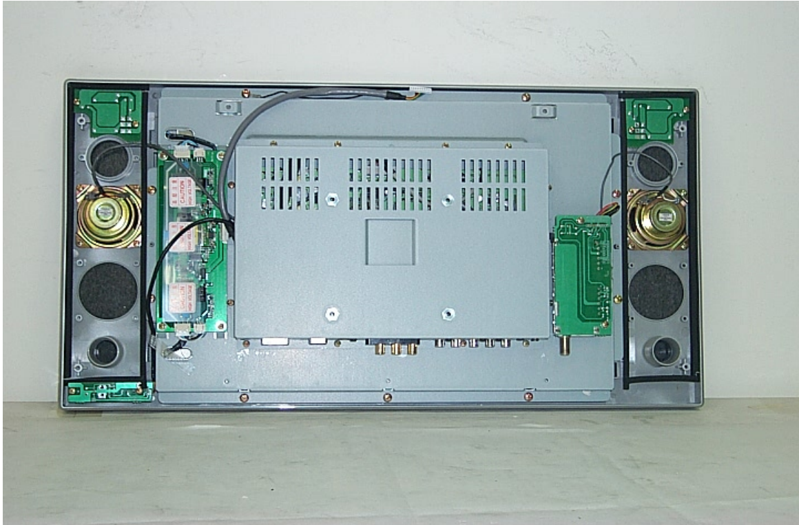
< Internal View – With Main Board Cover >
