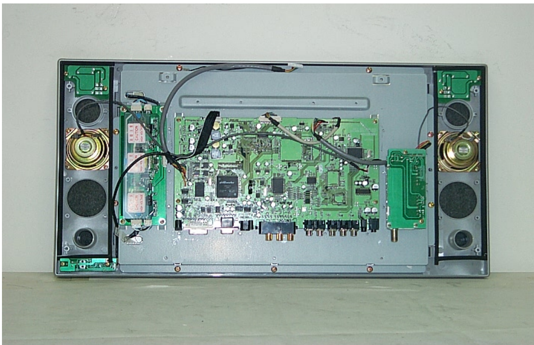
< Internal View - Without Main Board Cover >
