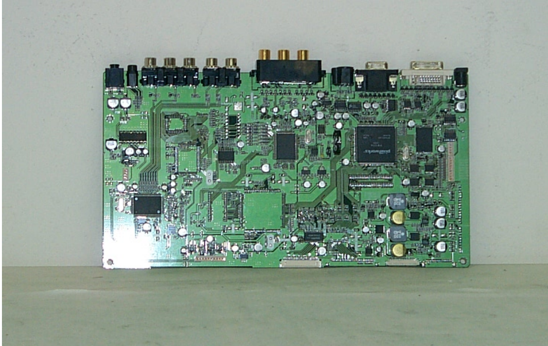
< Main Board – Top View >
