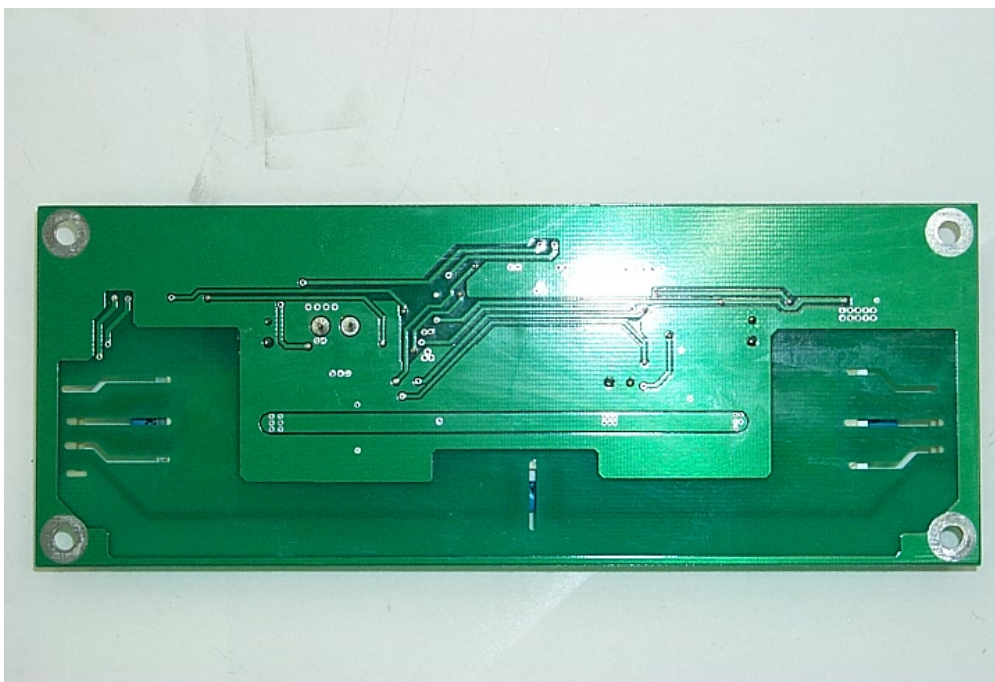
< Inverter Board – Bottom View >
