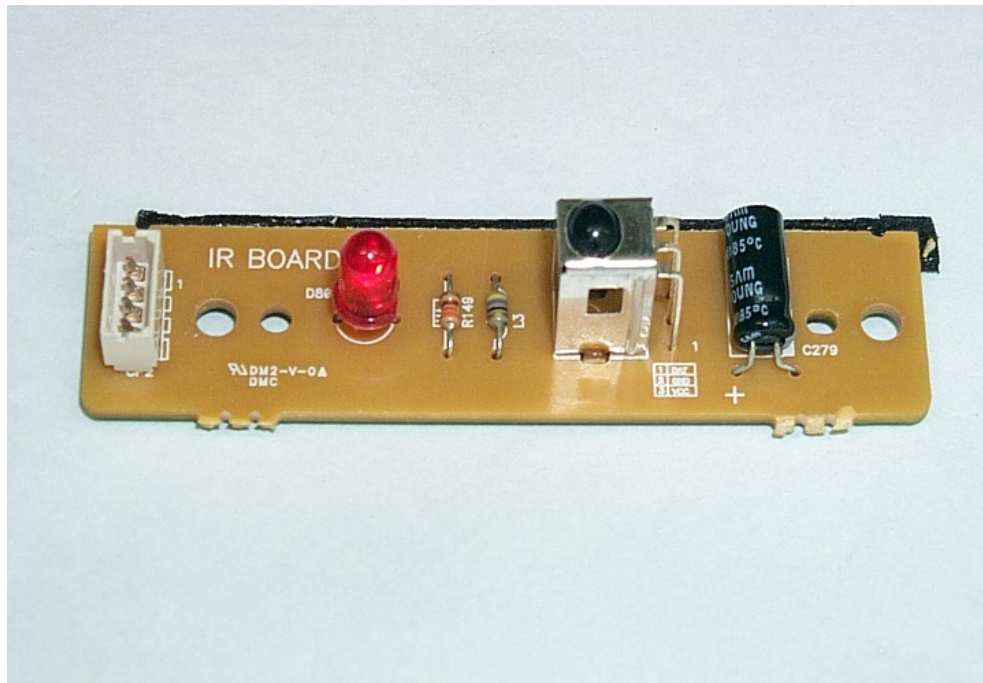
< IR Board – Top View >
