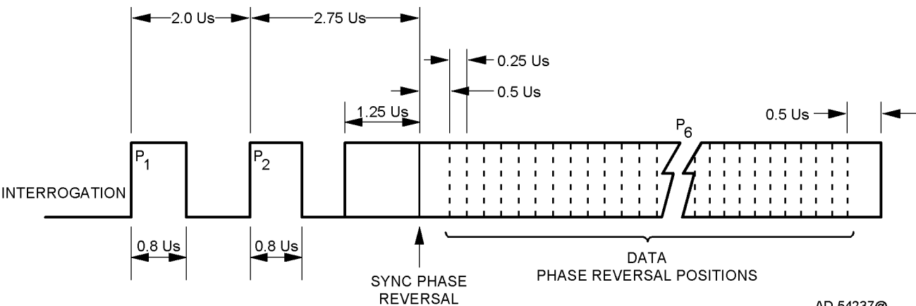
Figure 5. Mode S Pulse Format
