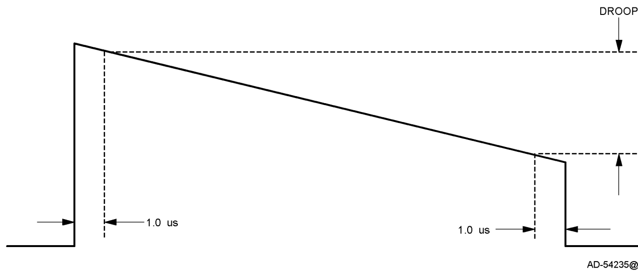
Figure 3. Pulse Droop Measurements
