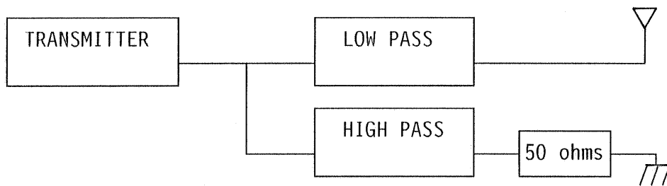
Harmonic Filter
