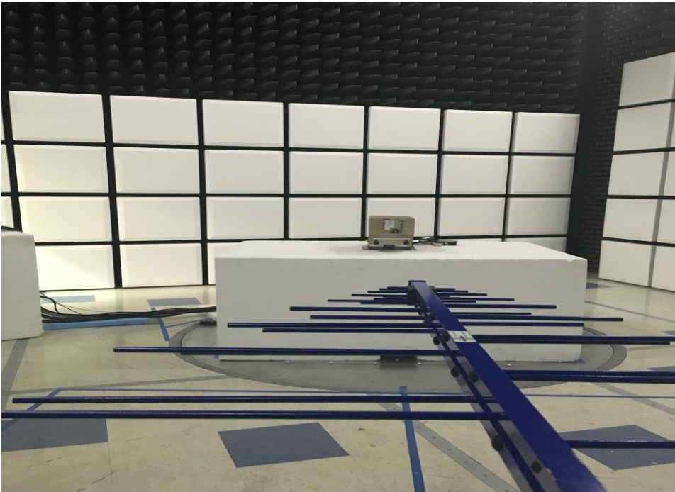
Radiated Testing 30Mhz-1Ghz
