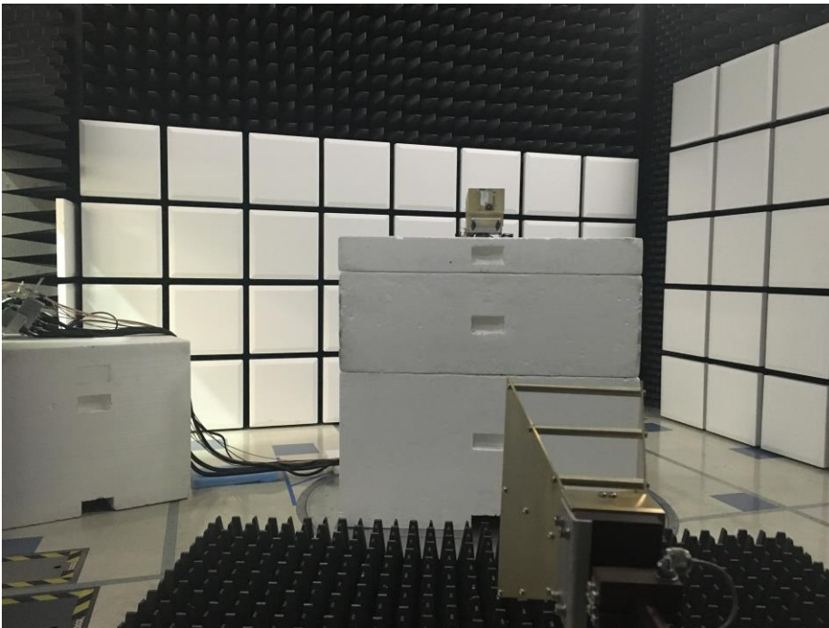
Radiated Testing 1-18Ghz
